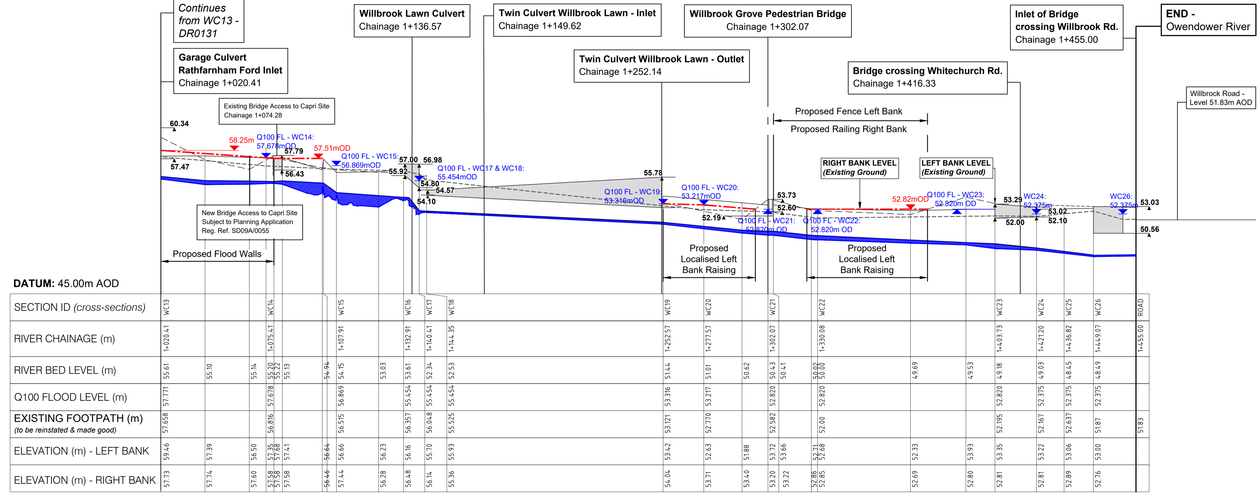
WHITECHURCH STREAM PROFILE - LONG SECTION / PROPOSED WORKS (2) Scale: Horiz. 1:1000, Vert. 1:200 @ A1
