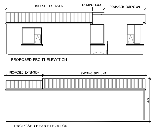
ELEVATIONS OF PROPOSED BAY NO.10 TO BELGARD PARK
