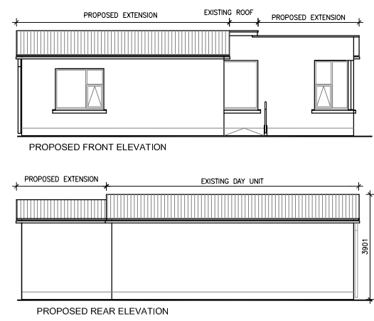
ELEVATIONS OF PROPOSED BAY NO.1 TO BELGARD PARK
