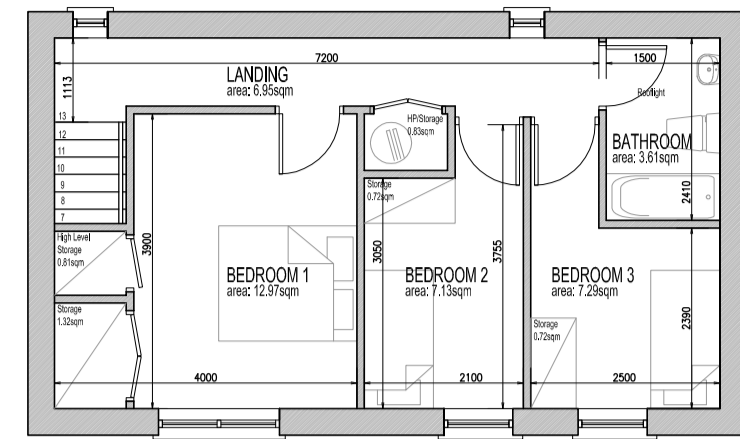
B4 - FIRST FLOOR PLAN SCALE- 1:100
