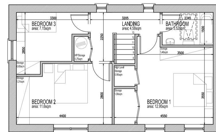
B5 - FIRST FLOOR PLAN SCALE- 1:100
