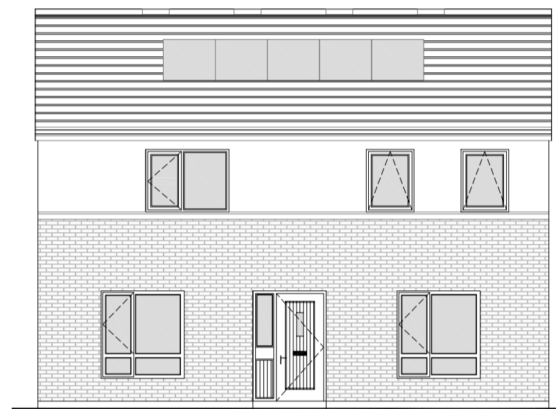
B5 - FRONT ELEVATION SCALE- 1:100
