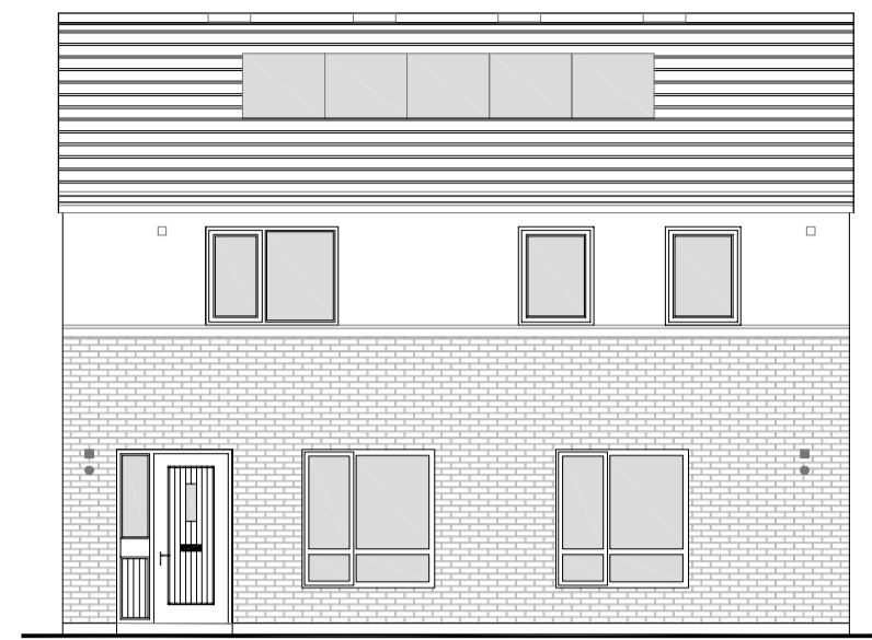
B4 - FRONT ELEVATION SCALE- 1:100
