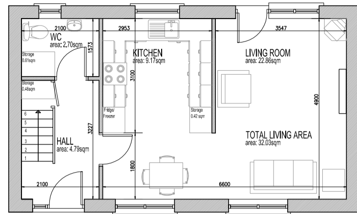
B4 - GROUND FLOOR PLAN SCALE- 1:100
