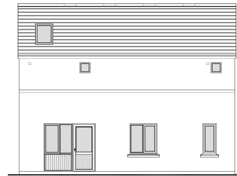
B4 - REAR ELEVATION SCALE- 1:100
