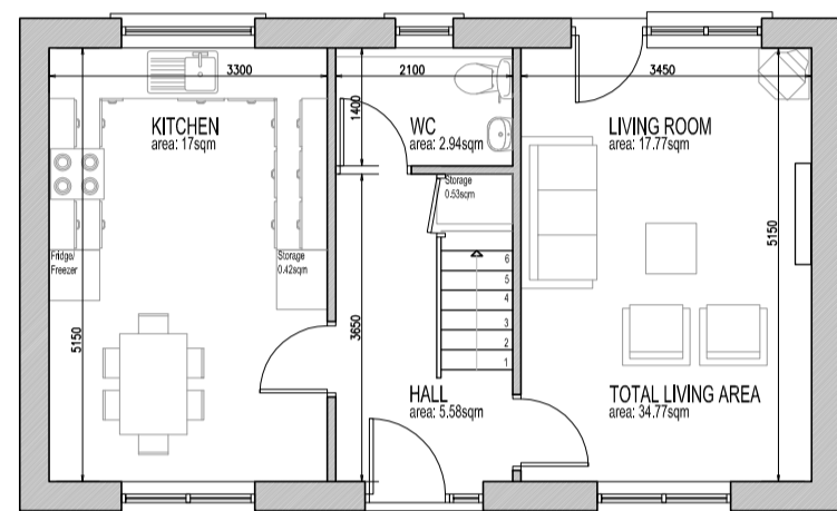
B5 - GROUND FLOOR PLAN SCALE- 1:100
