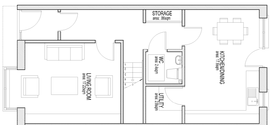
02 House Type T2 1:100 (A1)
