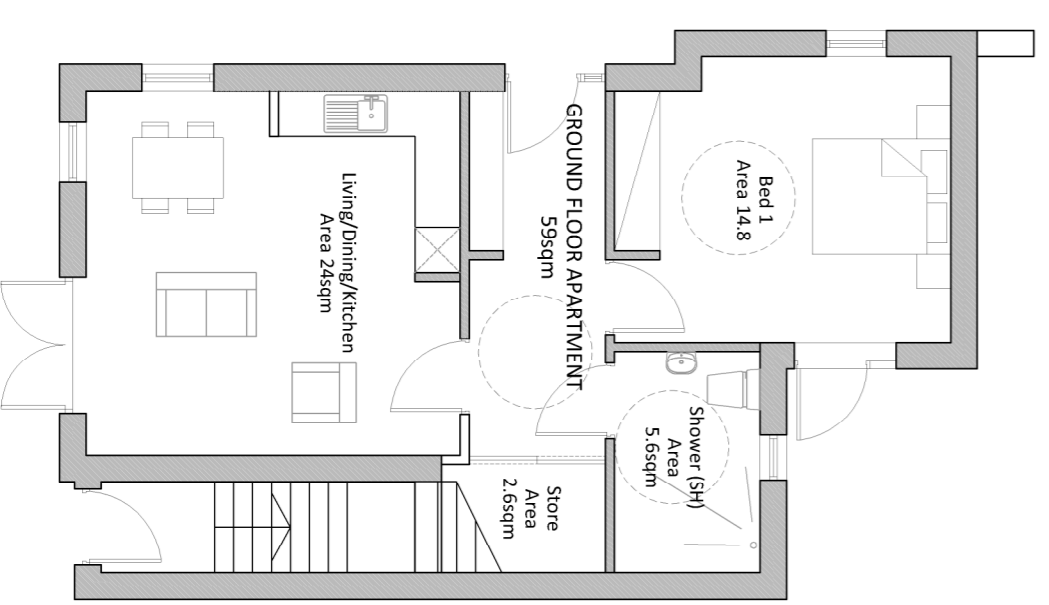
03 Duplex & Ground Floor Unit D2U 1:100 (A1)
