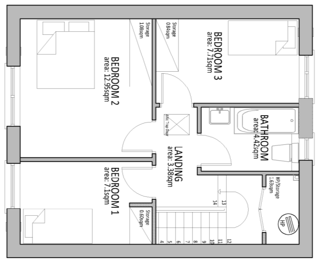
01 HOUSE TYPE K4 1:100 (A1)
