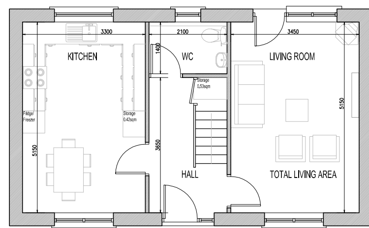
B5 - GROUND FLOOR PLAN
