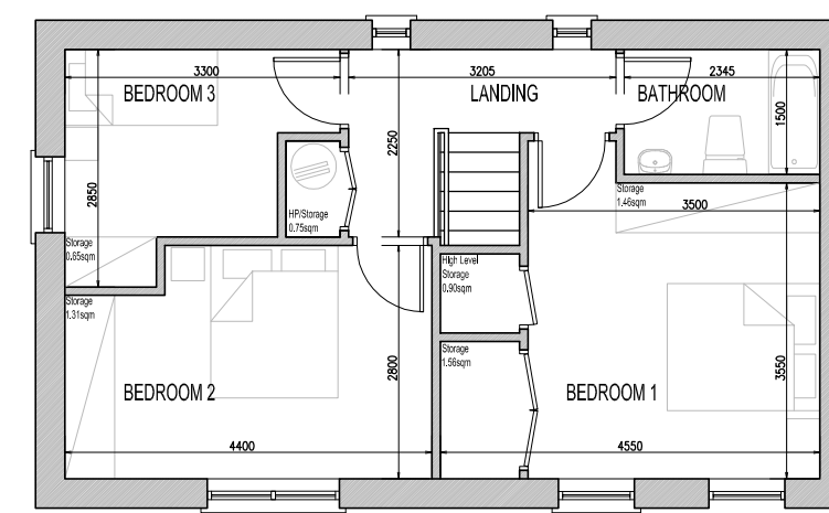
B5 - FIRST FLOOR PLAN
