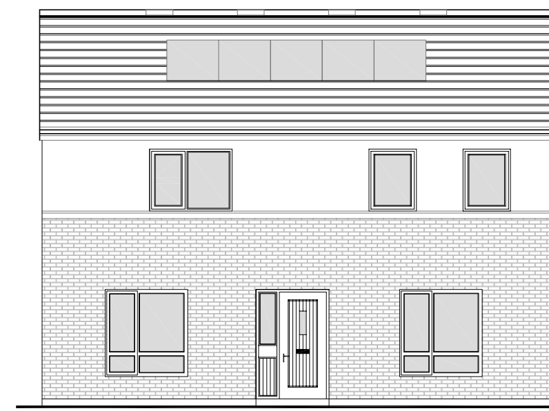
B5 - FRONT ELEVATION
