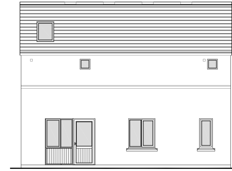
B4 - REAR ELEVATION
