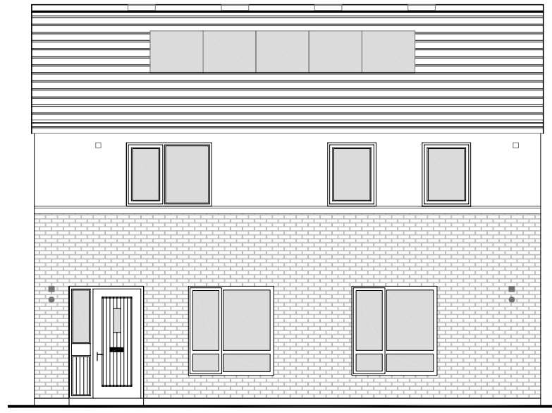
B4 - FRONT ELEVATION
