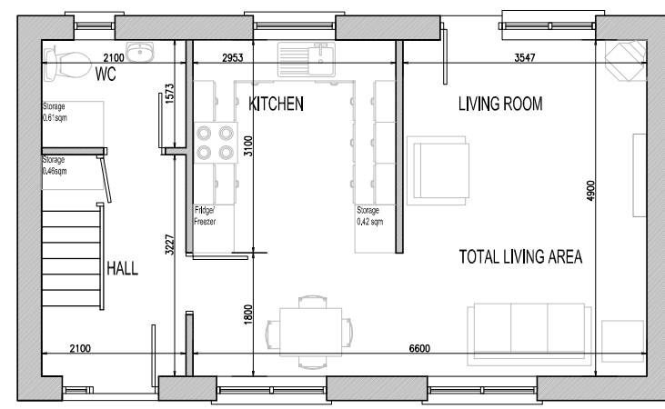
B4 - GROUND FLOOR PLAN
