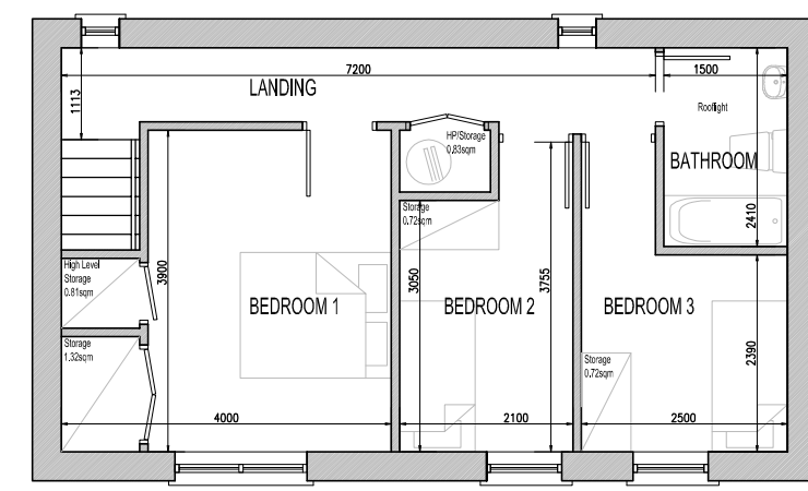
B4 - FIRST FLOOR PLAN
