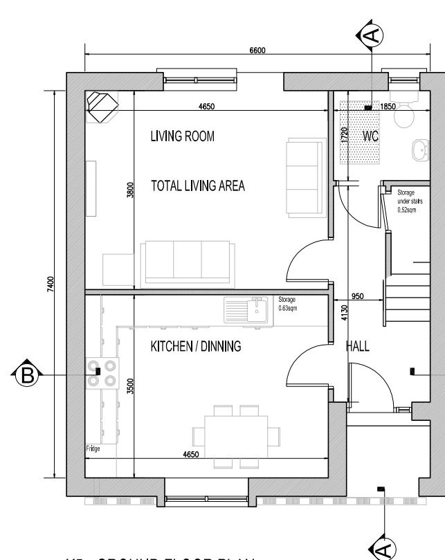
K5 - GROUND FLOOR PLAN
