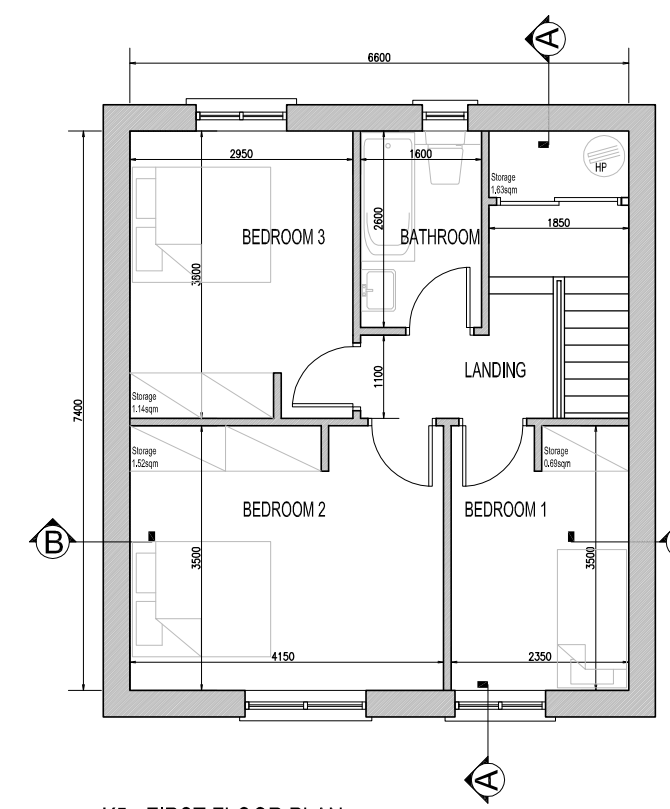
K5 - FIRST FLOOR PLAN
