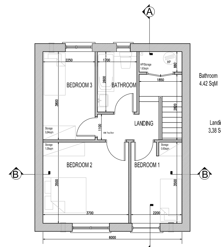
K4 - FIRST FLOOR PLAN
