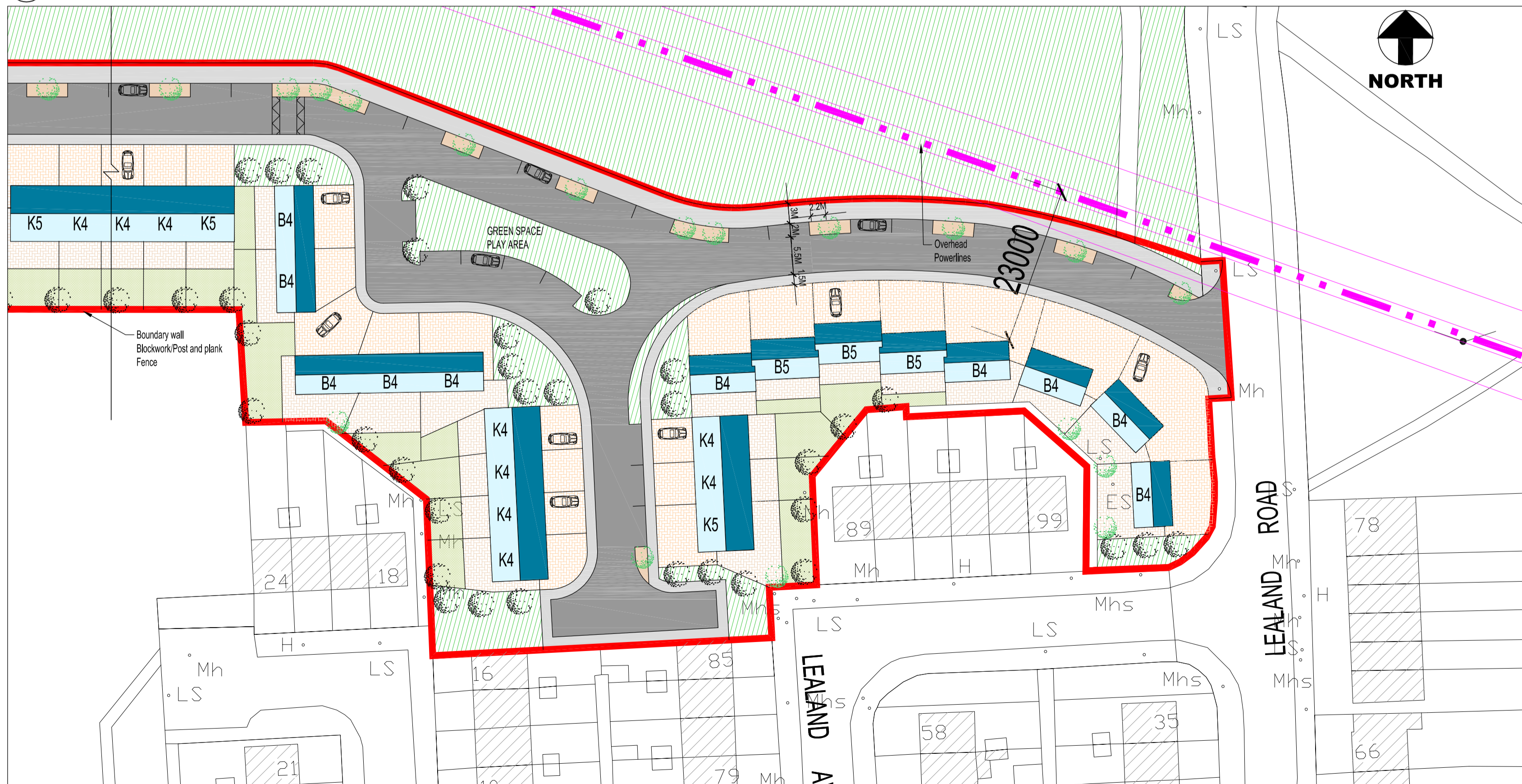
02 PROPOSED SITE PLAN- VIEW 2 1:500
