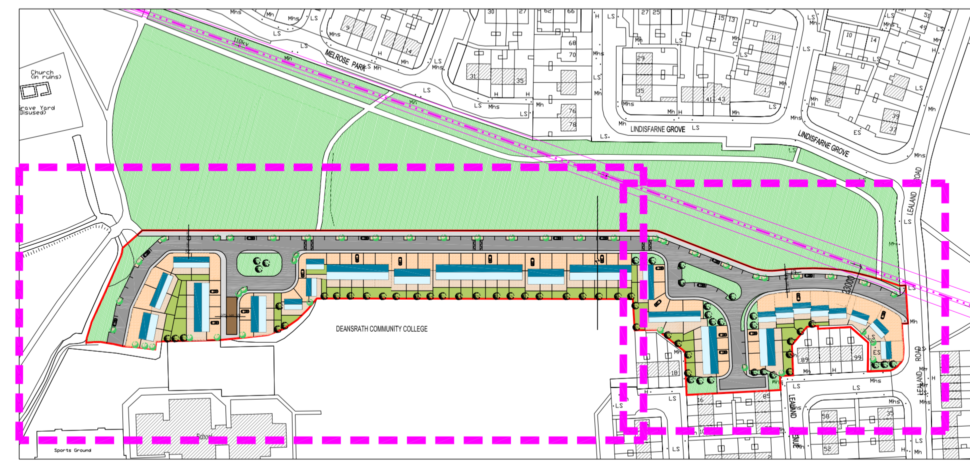
03 KEY PLAN 1:2000
