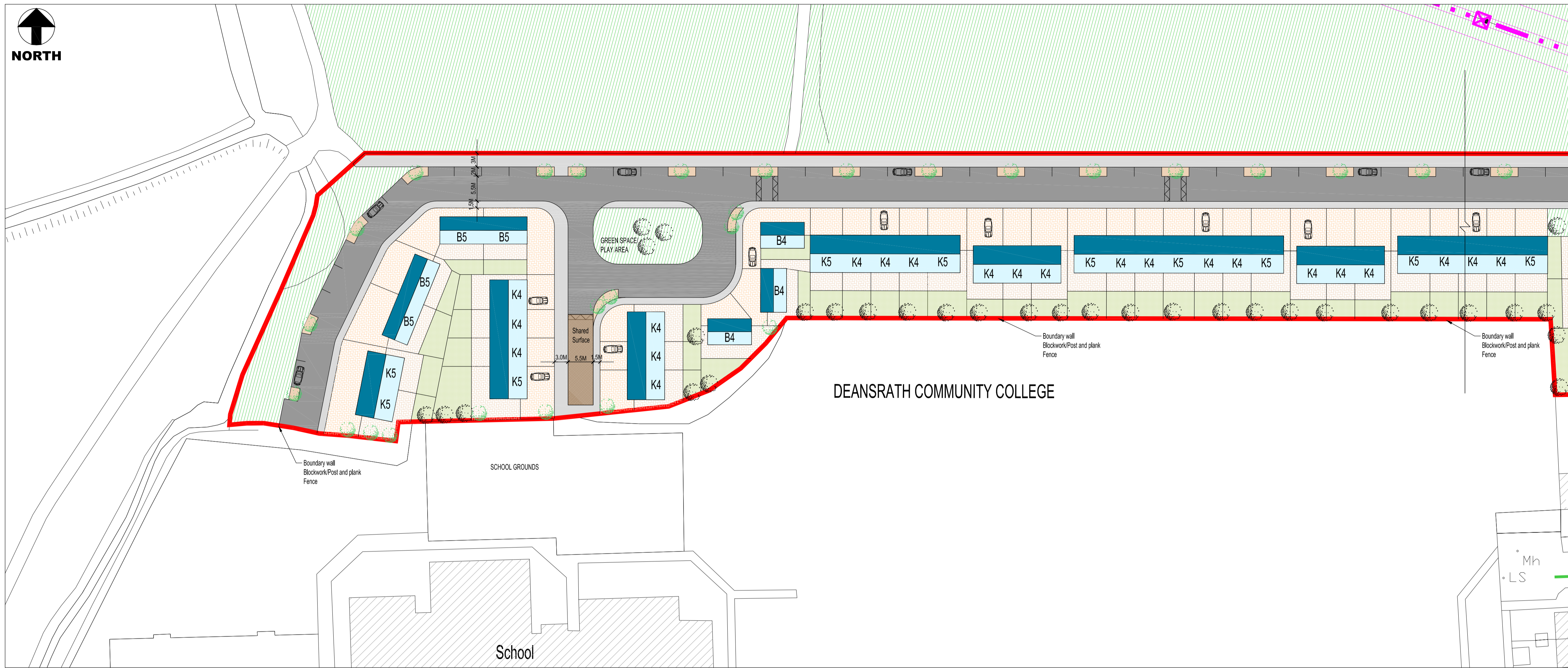
01 PROPOSED SITE PLAN- VIEW 1 1:500
