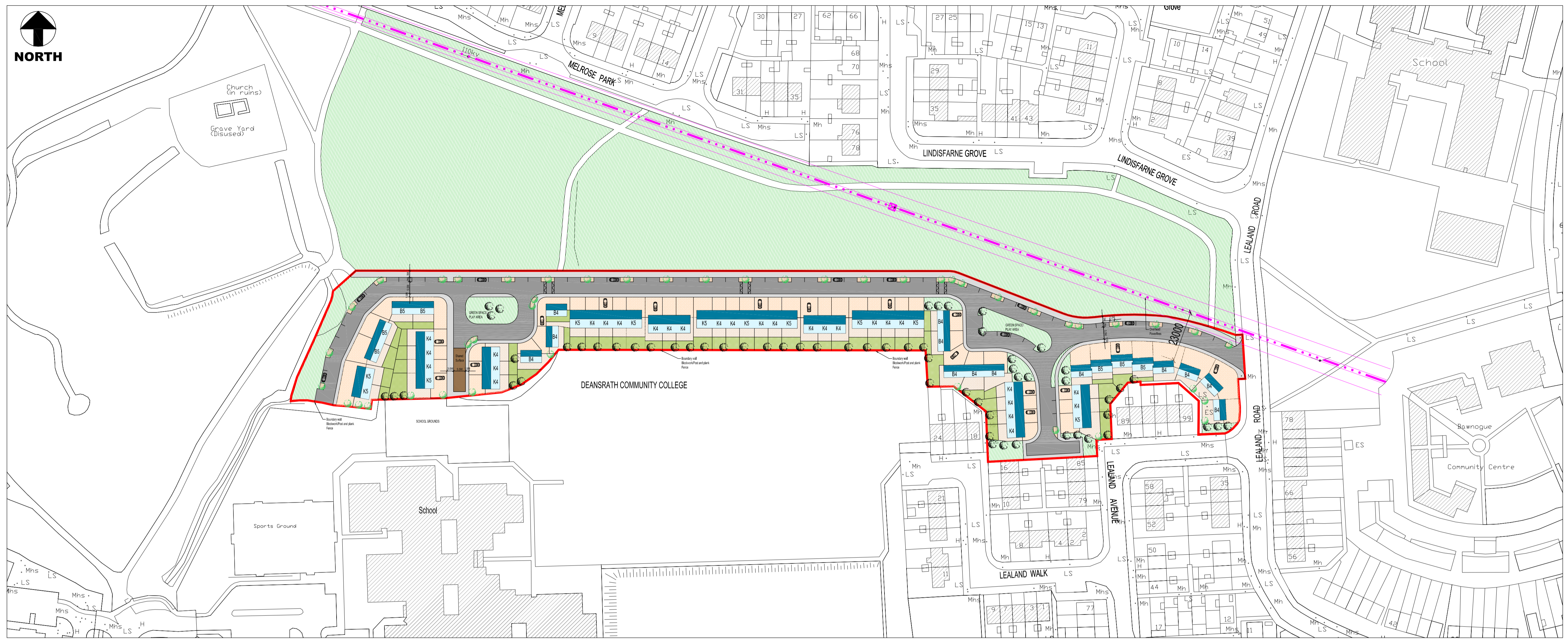
01 PROPOSED SITE PLAN 1:1000
