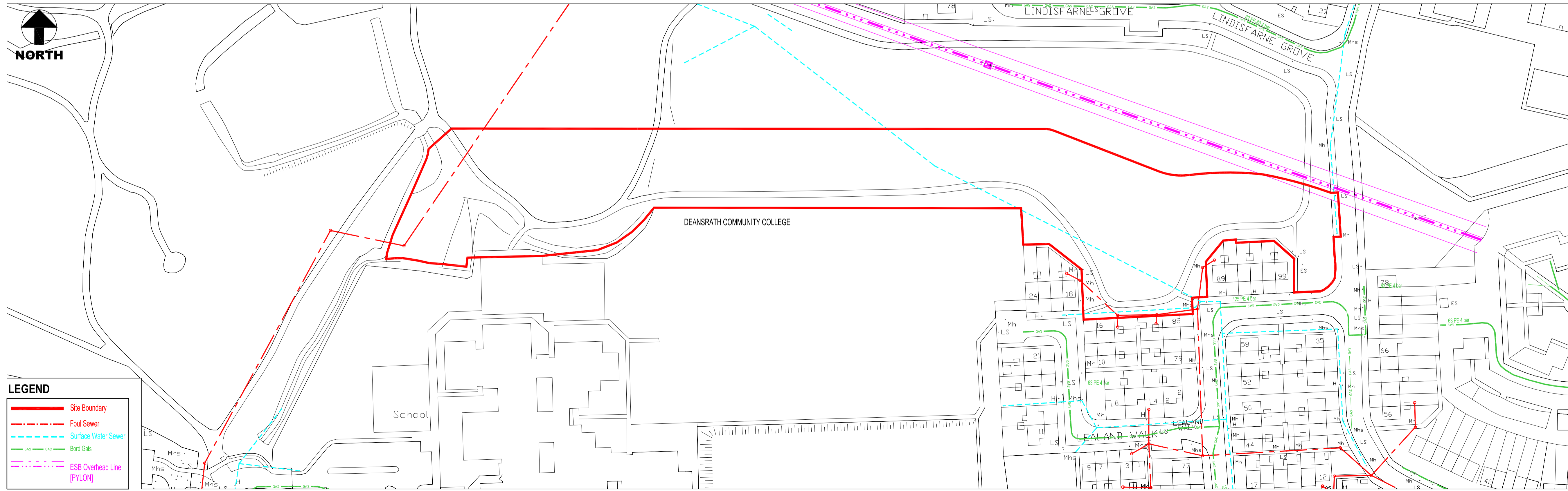
02 EXISTING SITE/CONTRANTS 1:1000
