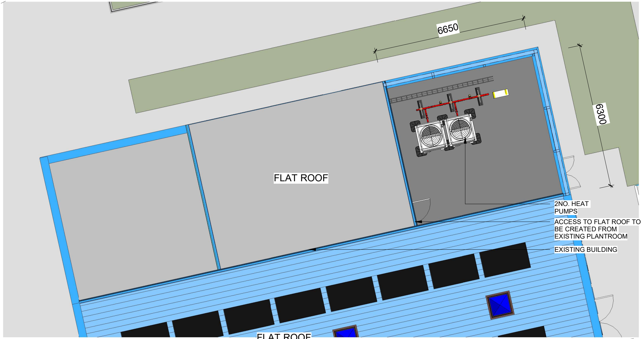
Civic Theatre - Site Plan (Detailed) 1 : 100
