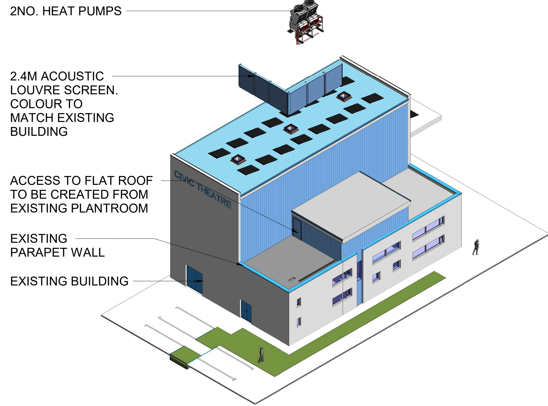
Civic Theatre - Perspective View
