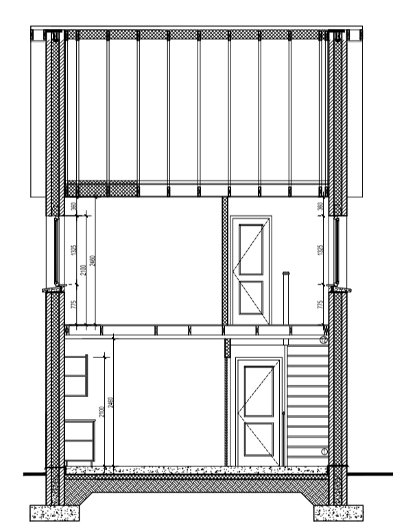
HOUSE TYPE N4- SECTION B-B 1:100
