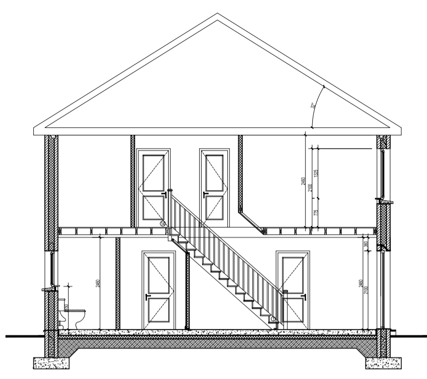
HOUSE TYPE N5- SECTION A-A 1:100
