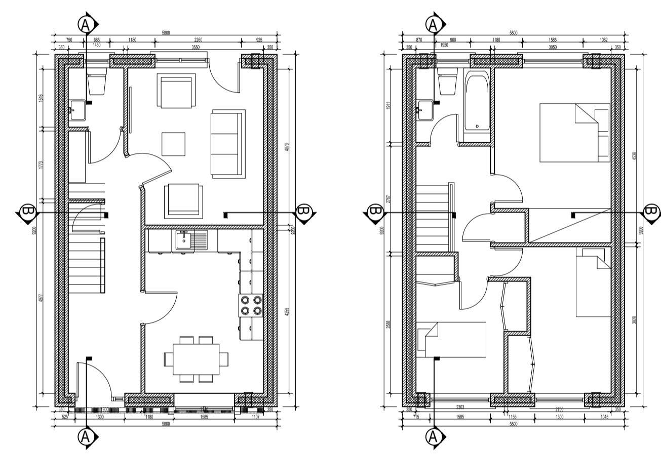
HOUSE TYPE N4- GF PLAN 1:100
