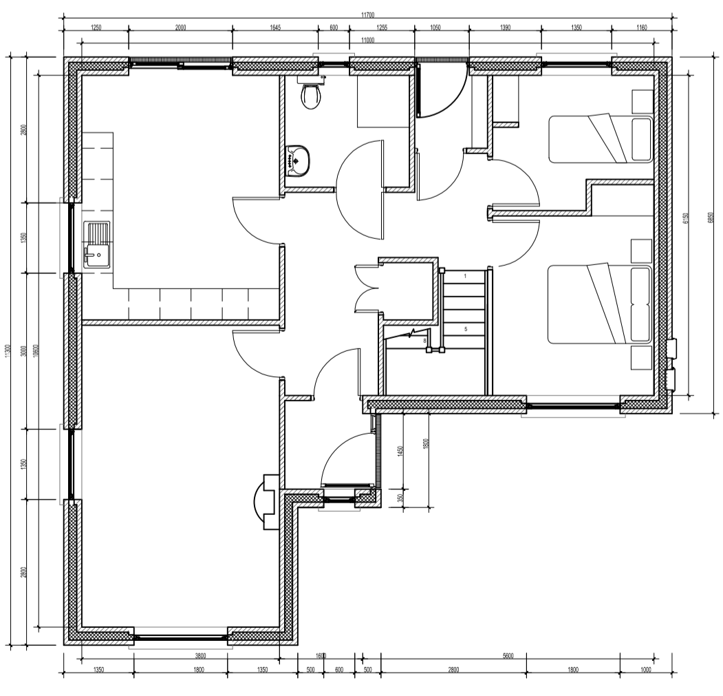
HOUSE TYPE T7- GF PLAN 1:100
