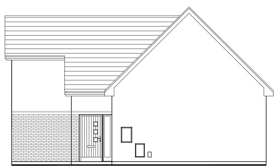
HOUSE TYPE T7- FRONT ELEVATION 1:100
