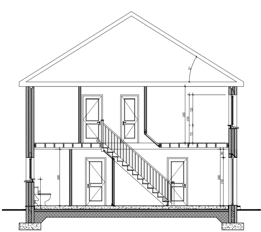
HOUSE TYPE N4- SECTION A-A 1:100
