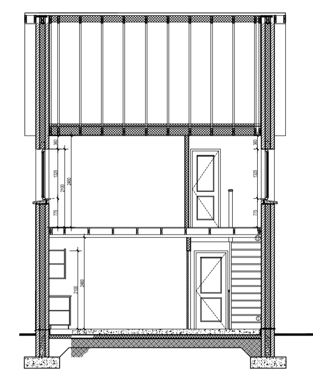
HOUSE TYPE N5- SECTION B-B 1:100
