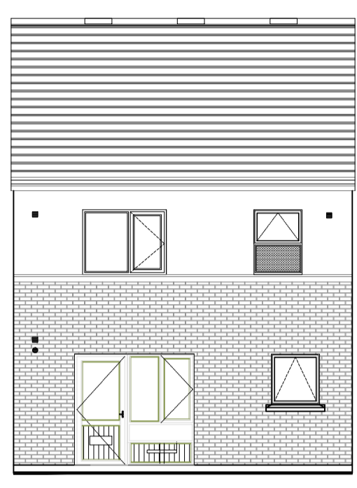
HOUSE TYPE N5- REAR ELEVATION 1:100
