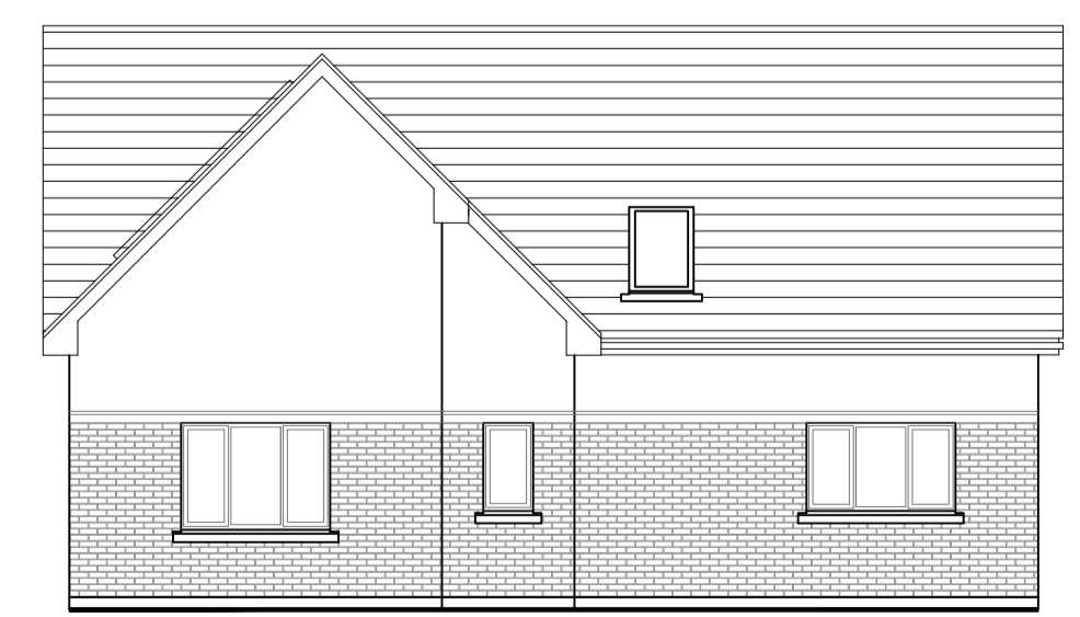
HOUSE TYPE T7- REAR ELEVATION 1:100
