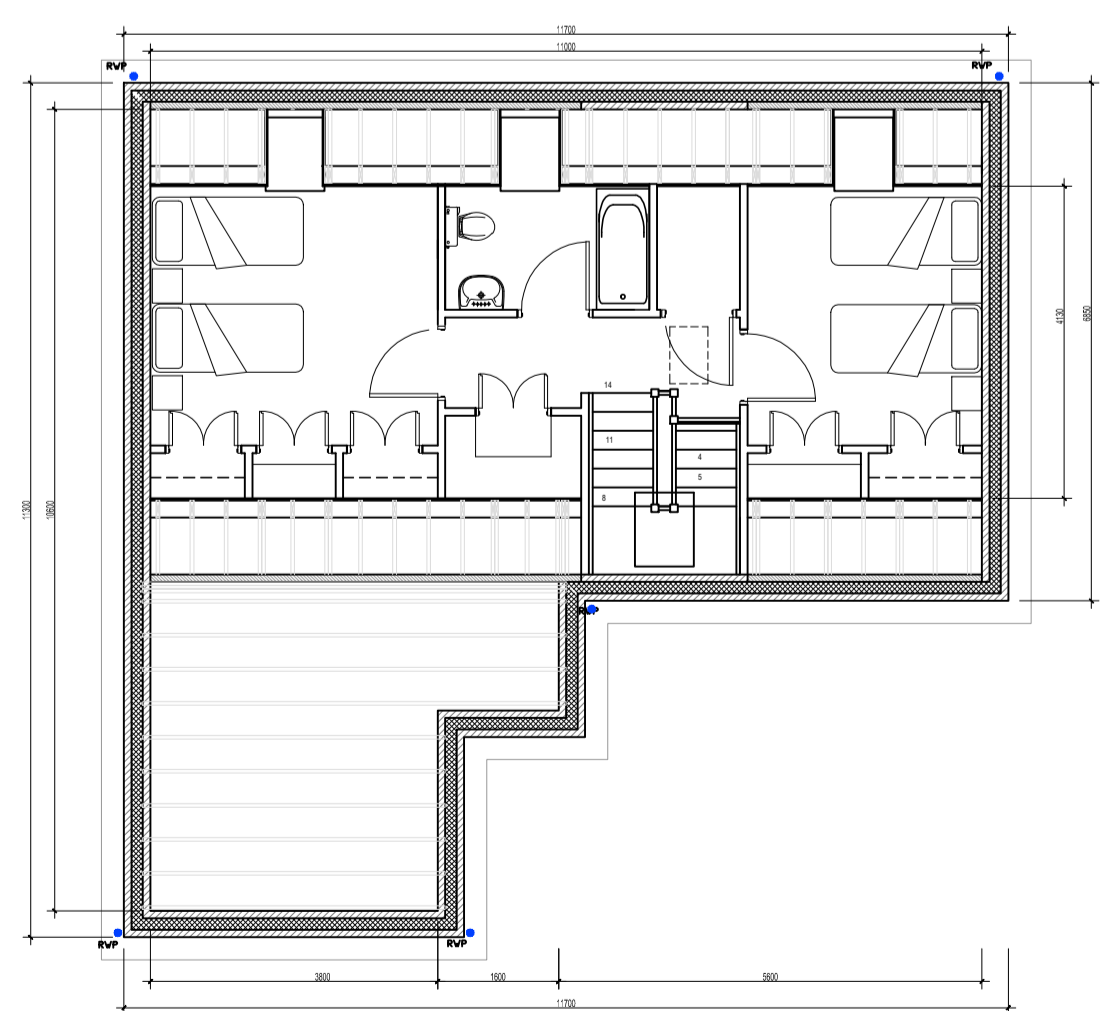
HOUSE TYPE T7- FF PLAN 1:100
