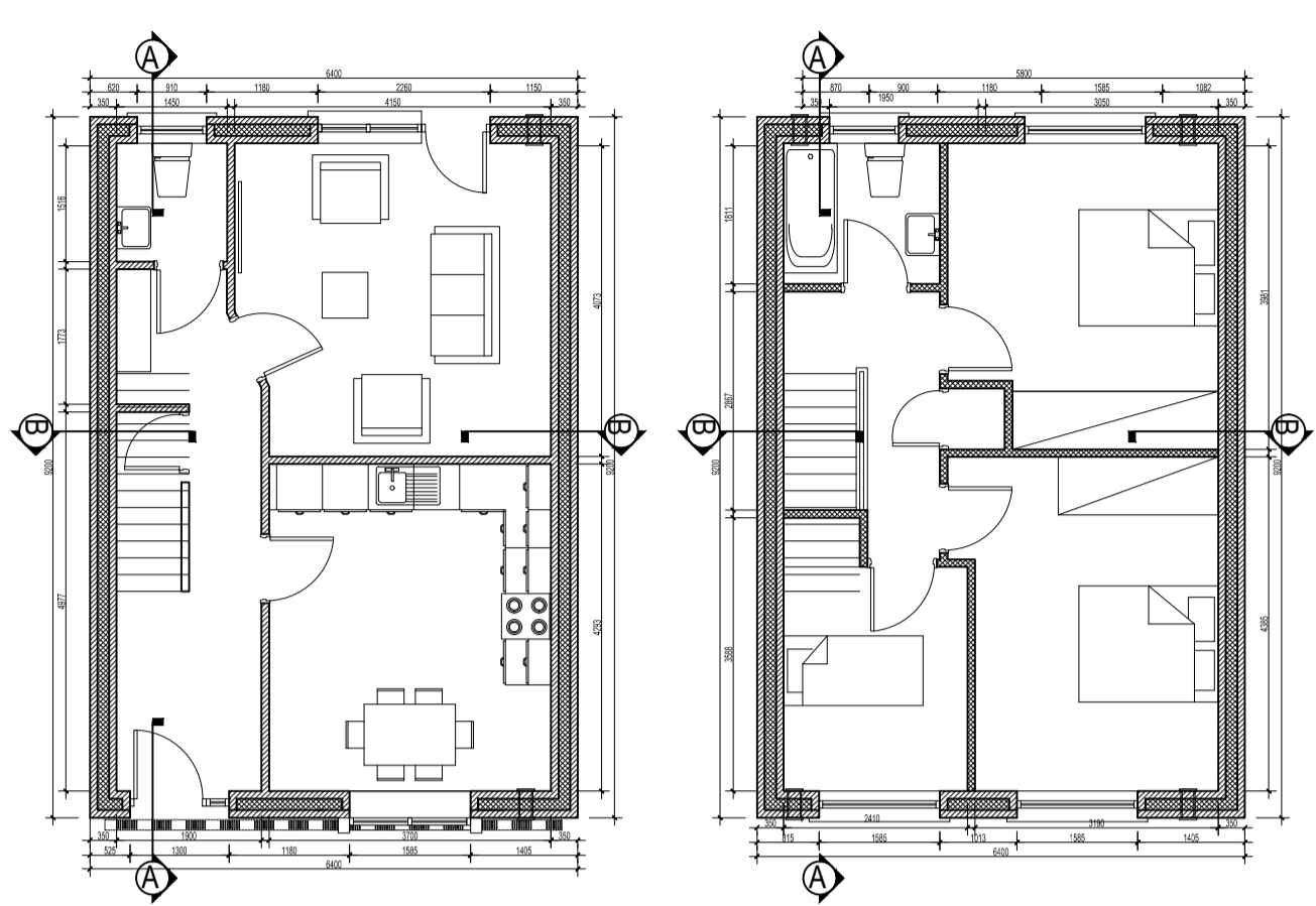
HOUSE TYPE N5- GF PLAN 1:100
