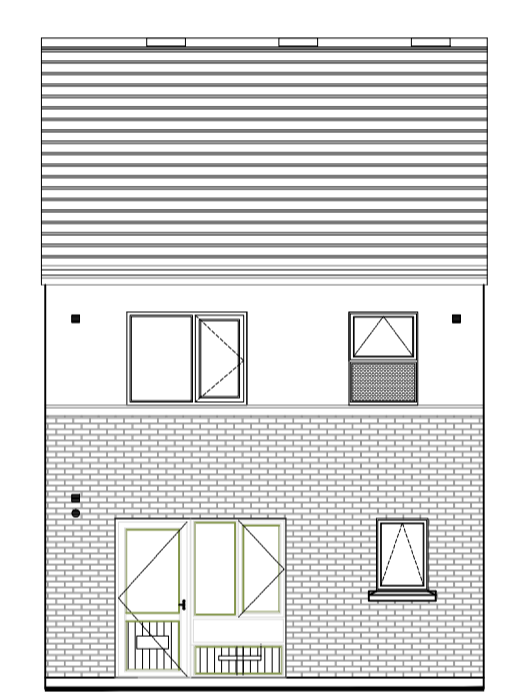
HOUSE TYPE N4- REAR ELEVATION 1:100
