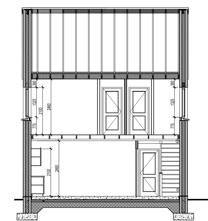
HOUSE TYPE K5- SECTION B-B 1:100
