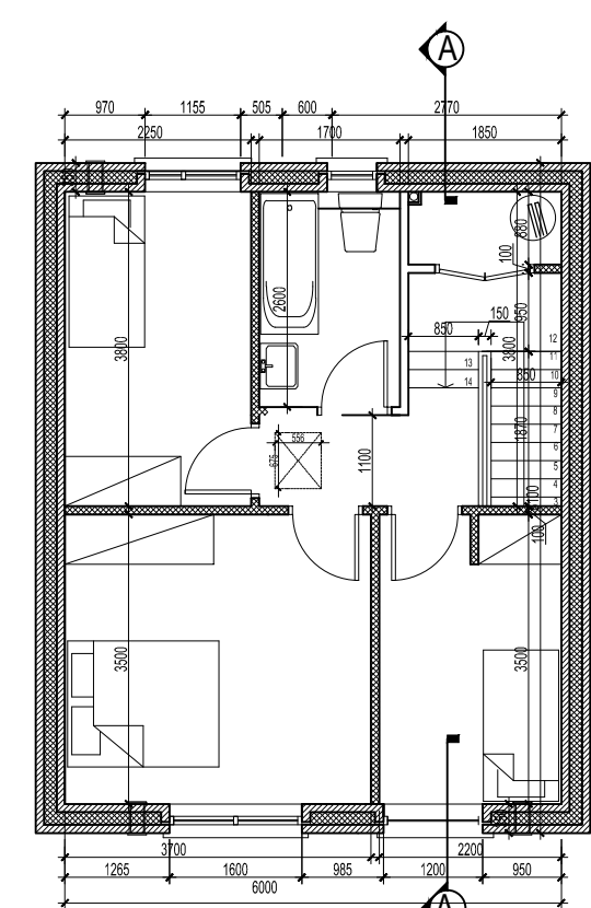
HOUSE TYPE K4- FF PLAN 1:100
