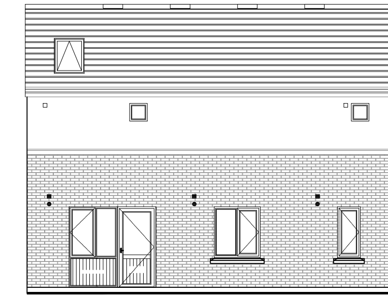
HOUSE TYPE B4- REAR ELEVATION 1:100
