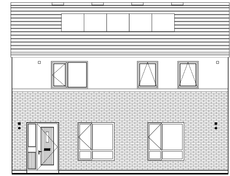
HOUSE TYPE B4- FRONT ELEVATION 1:100
