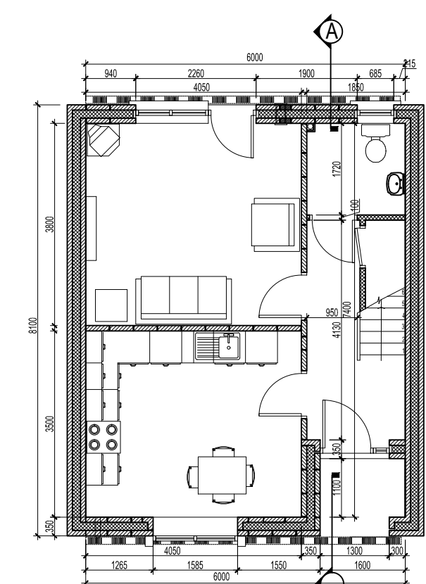
HOUSE TYPE K4- GF PLAN 1:100
