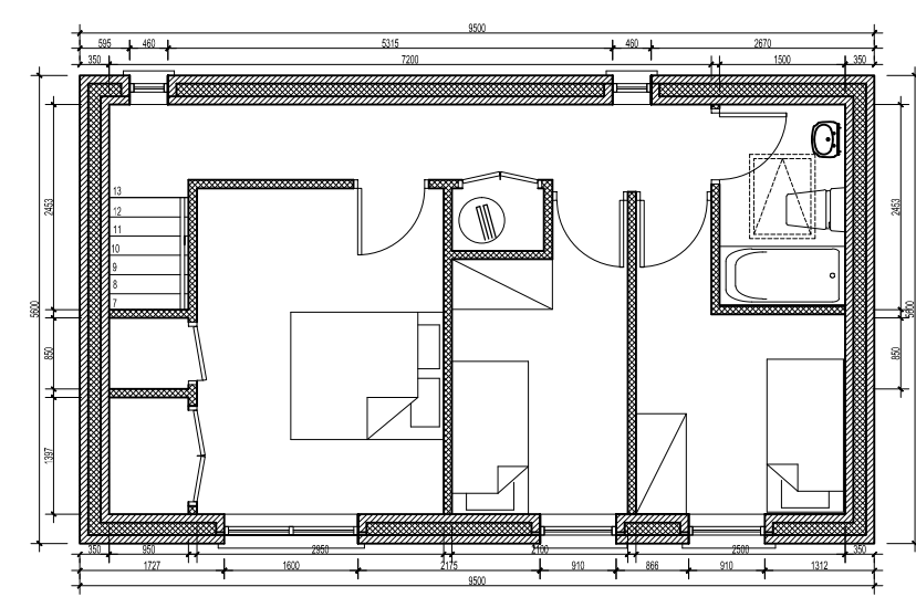
HOUSE TYPE B4- FF PLAN 1:100
