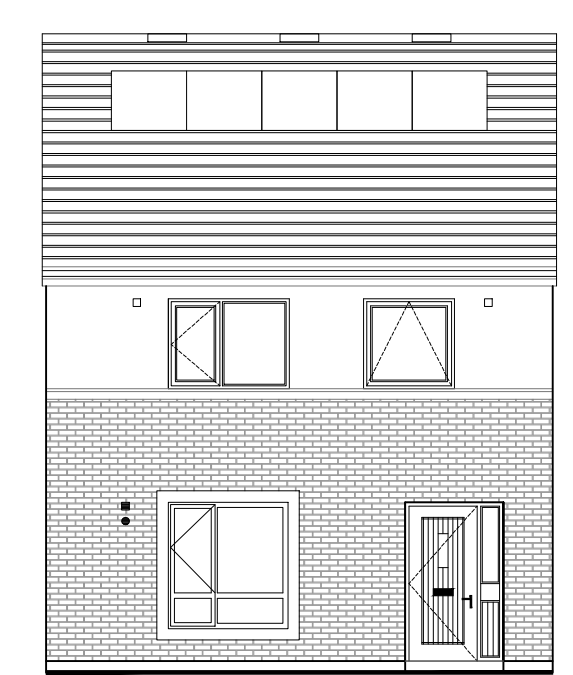
HOUSE TYPE K4- FRONT ELEVATION 1:100
