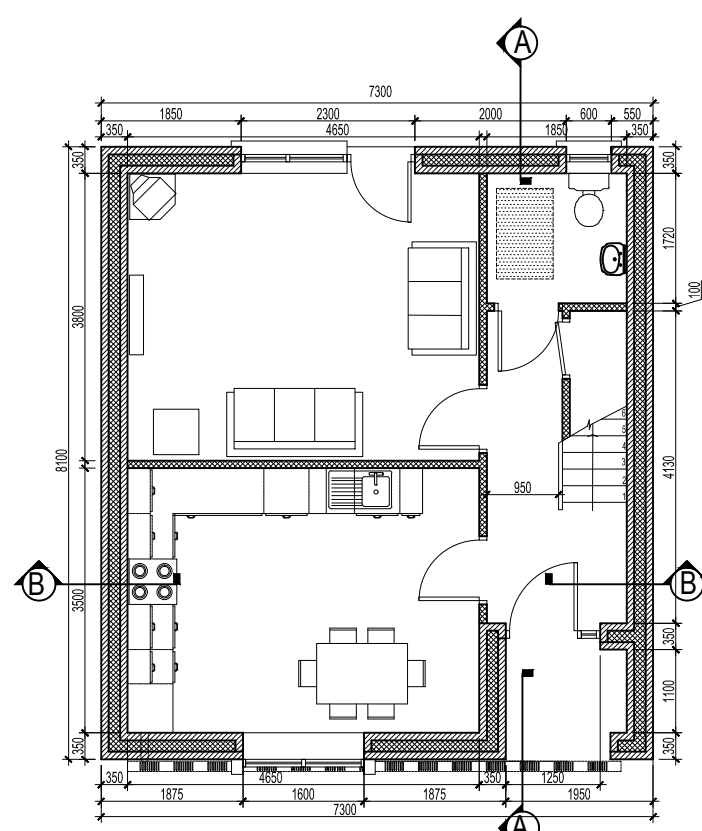
HOUSE TYPE K5- GF PLAN 1:100
