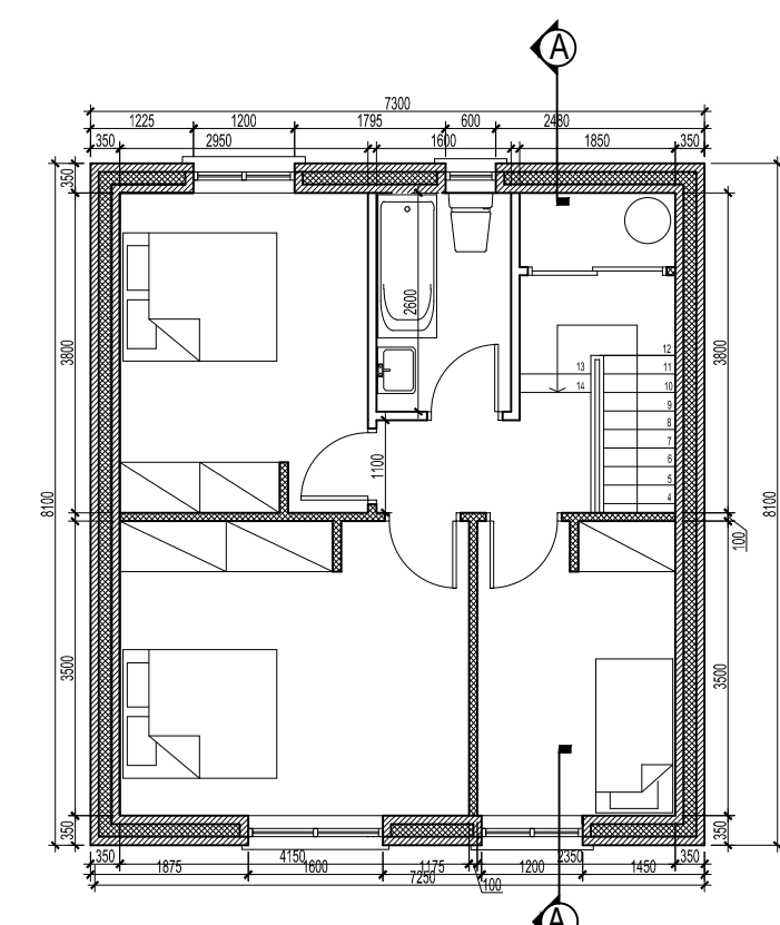
HOUSE TYPE K5- FF PLAN 1:100
