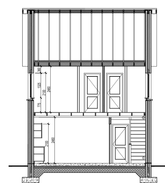
HOUSE TYPE K- SECTION B-B 1:100
