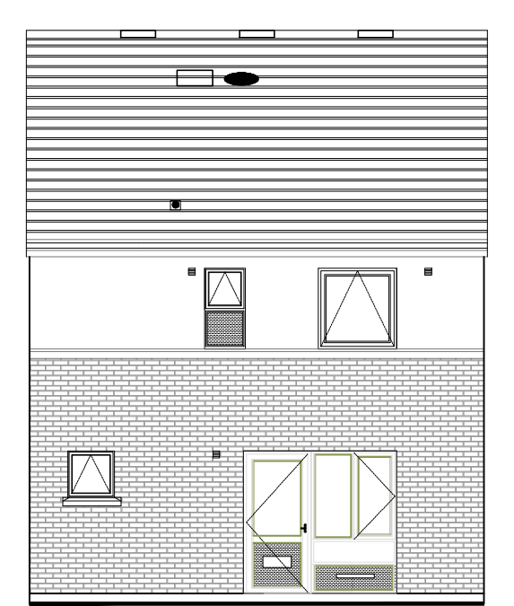
HOUSE TYPE K4- REAR ELEVATION 1:100
