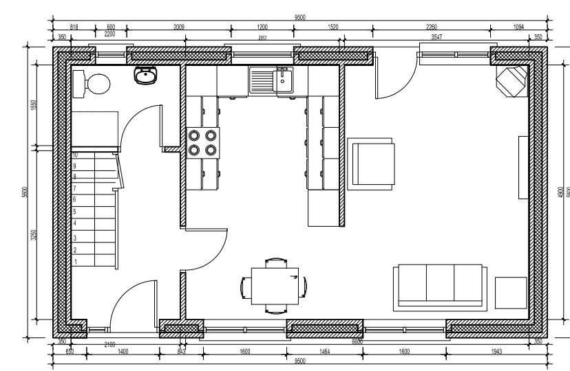
HOUSE TYPE B4- GF PLAN 1:100
