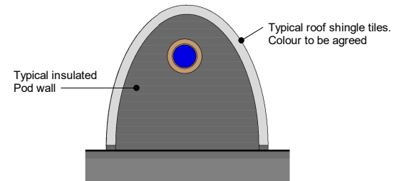
4 TYPICAL POD REAR ELEVATION 1 : 100
