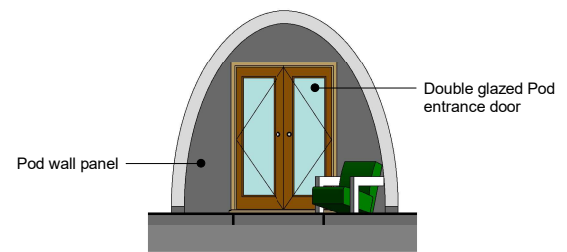
2 TYPICAL POD FRONT ELEVATION 1 : 100
