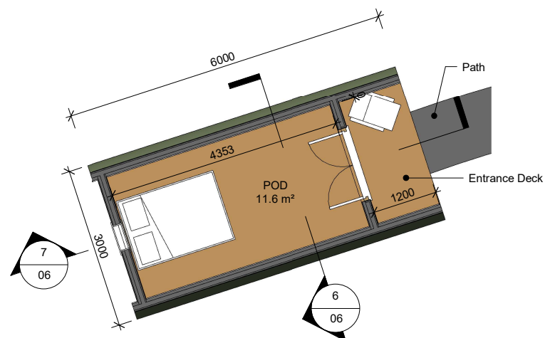
5 TYPICAL GLAMPING POD PLAN 1 : 100
