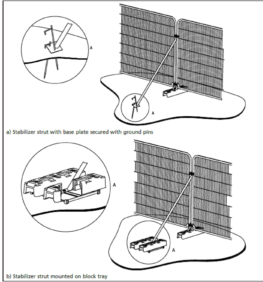
Tree protection fence typical detail
