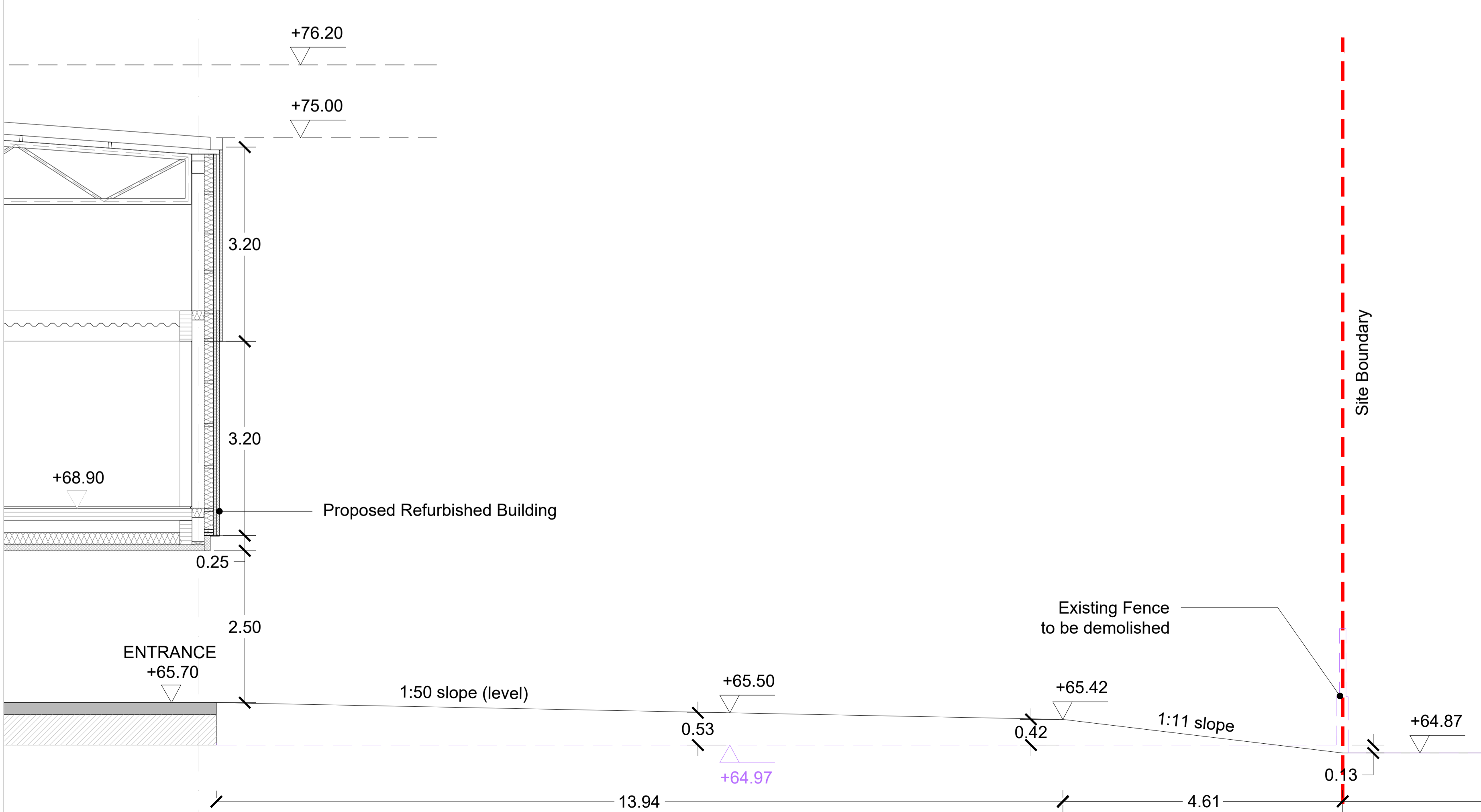
Proposed Landscape Section 03 Scale 1:50
