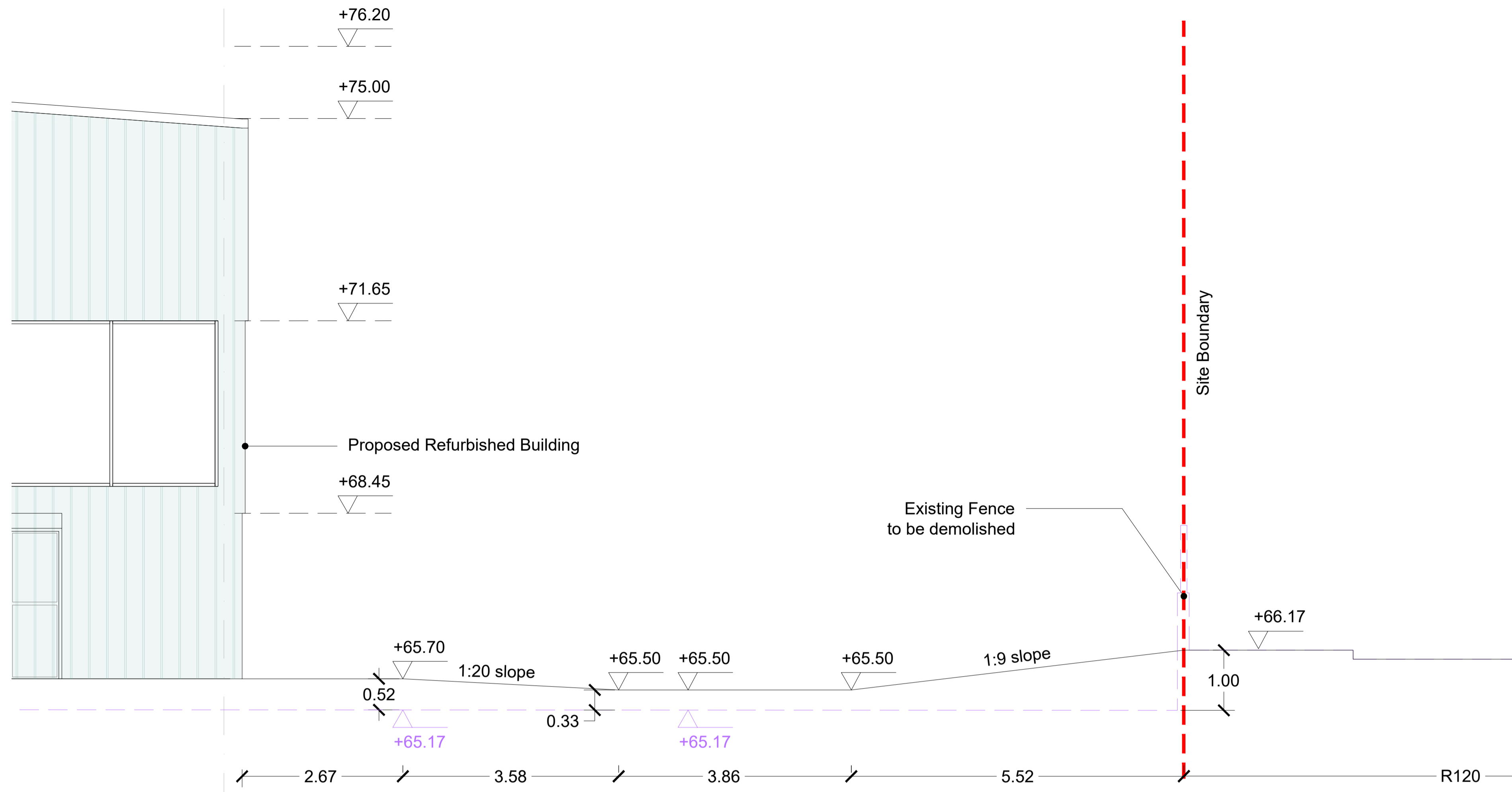
Proposed Landscape Section 01 Scale 1:50
