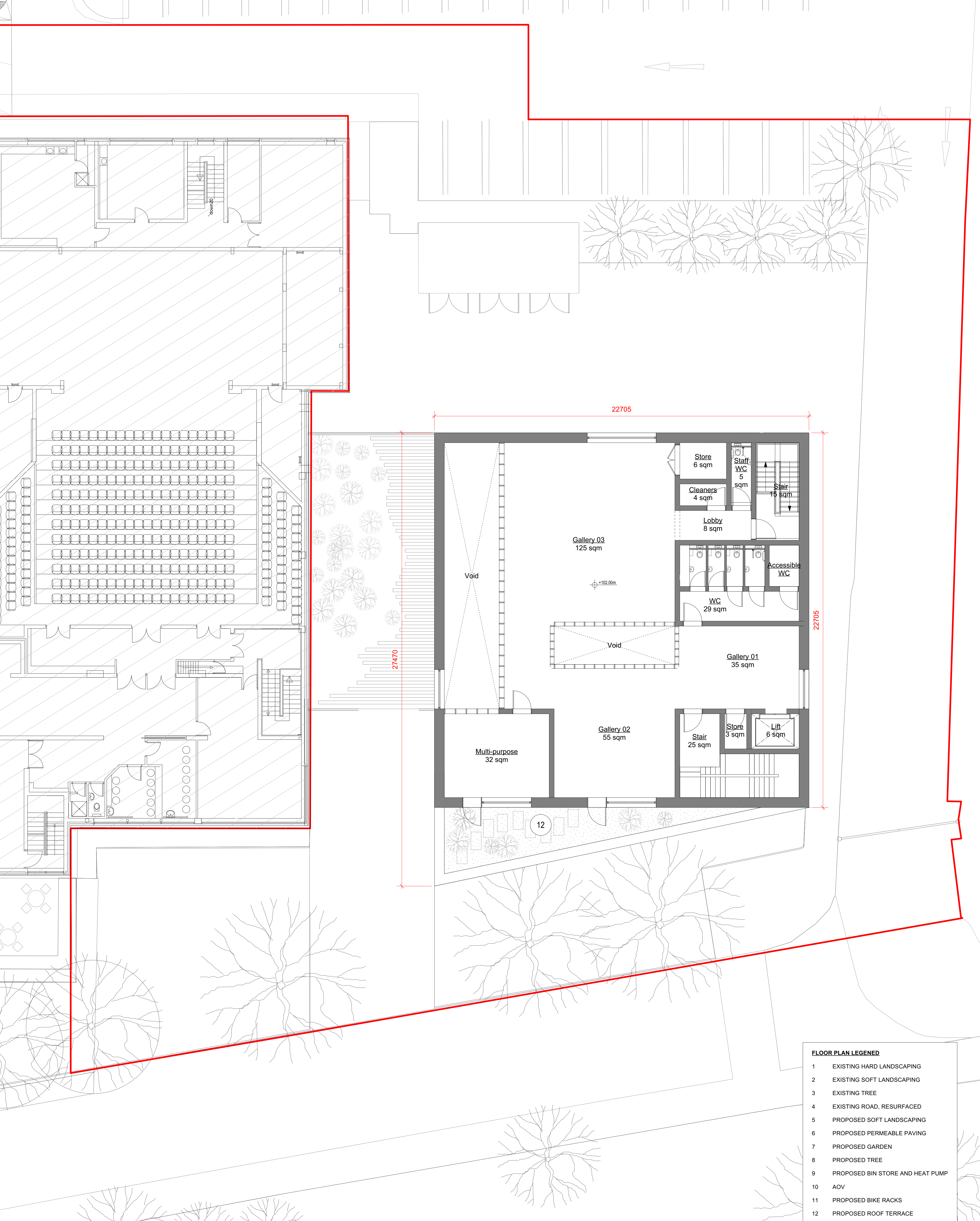
01 First Floor Plan - Proposed 101 Scale 1:100 @ A1
