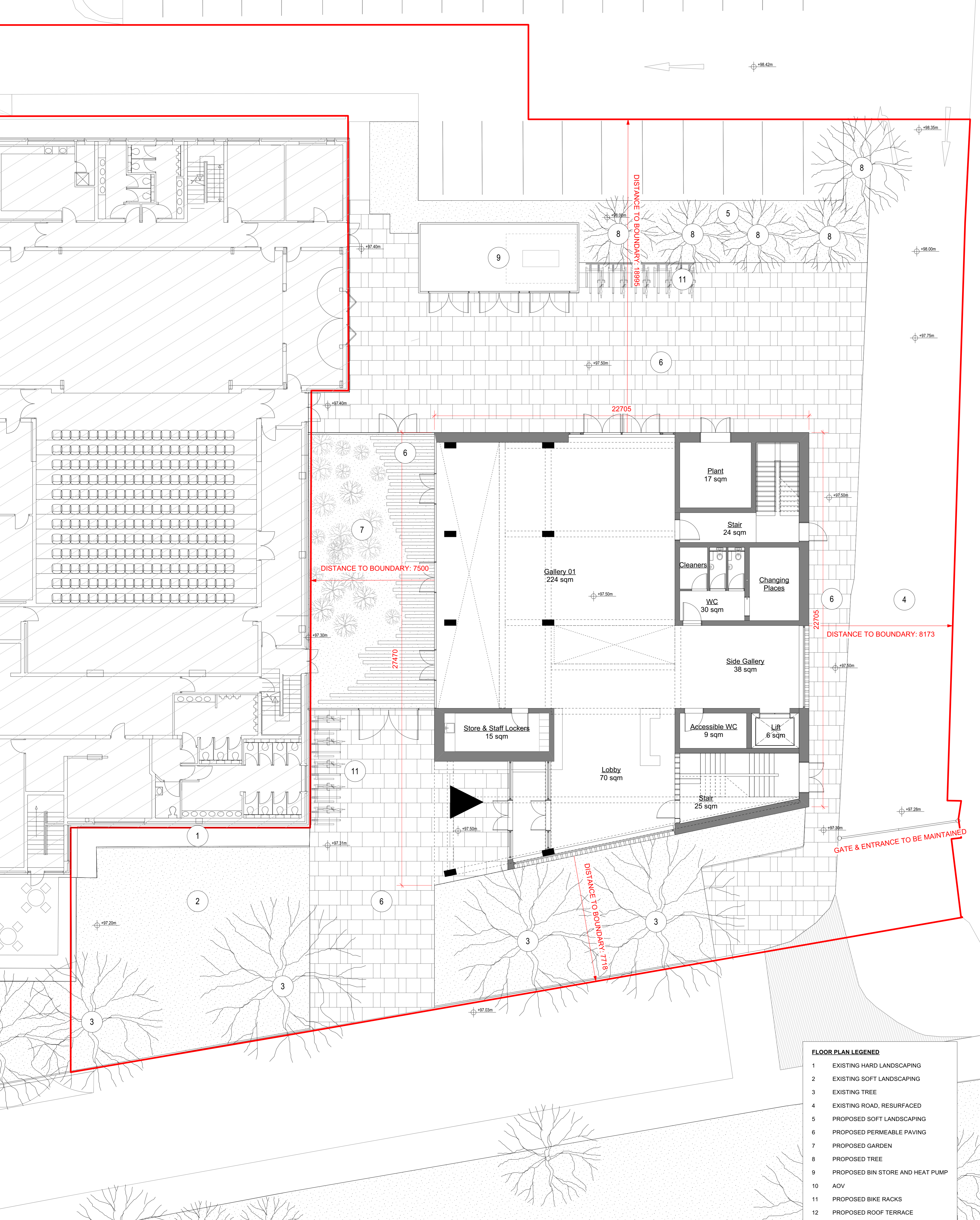
01 Ground Floor Plan - Proposed 100 Scale 1:100 @ A1
