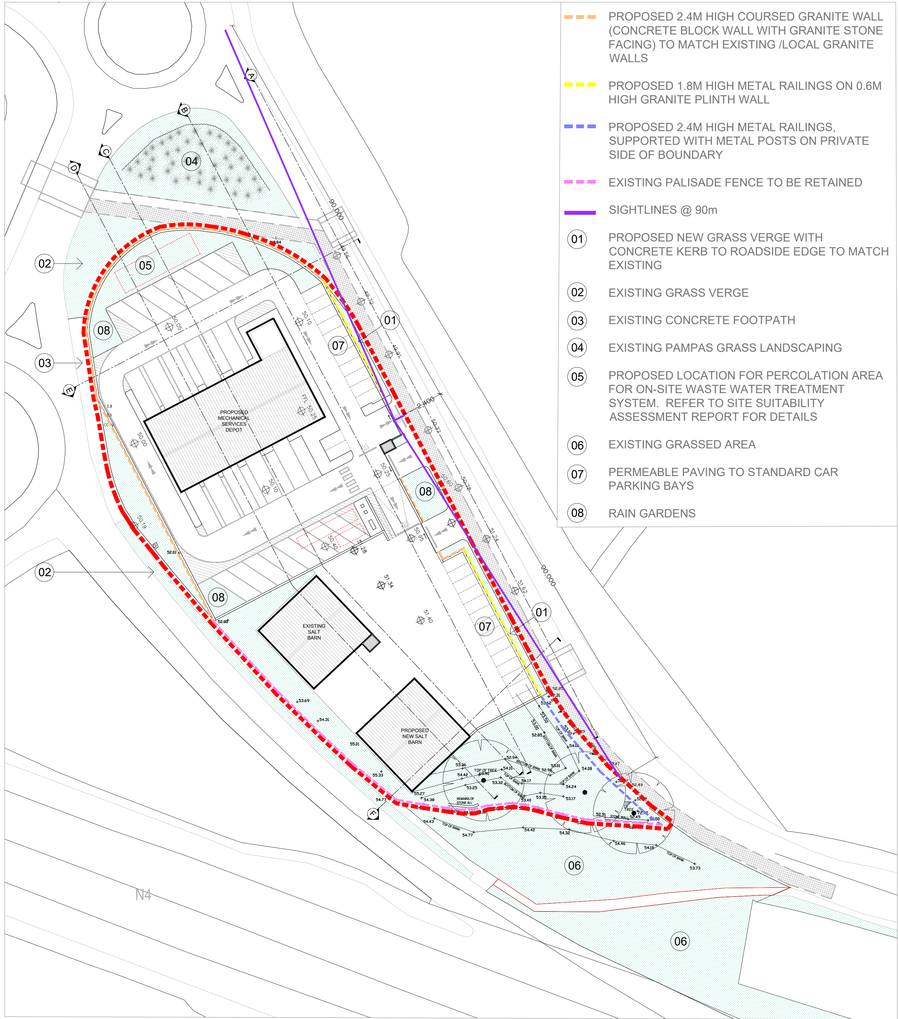
01 P01 PROPOSED SITE LANDSCAPING LAYOUT PLAN SCALE = 1:500 @A1, 1:1000@A3
