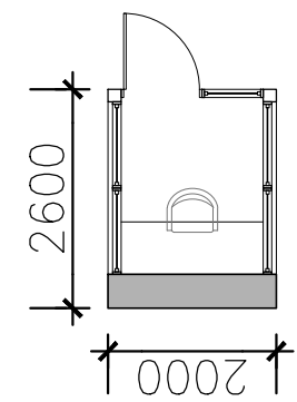
04 P01 PROPOSED PLAN SCALE = 1:100 @A1, 1:200@A3
