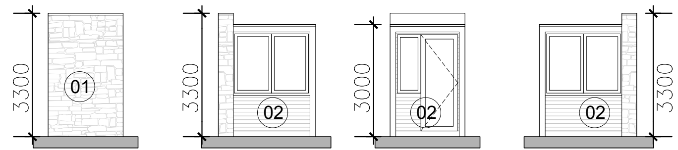
03 P01 PROPOSED ELEVATIONS SCALE = 1:100 @A1, 1:200@A3
