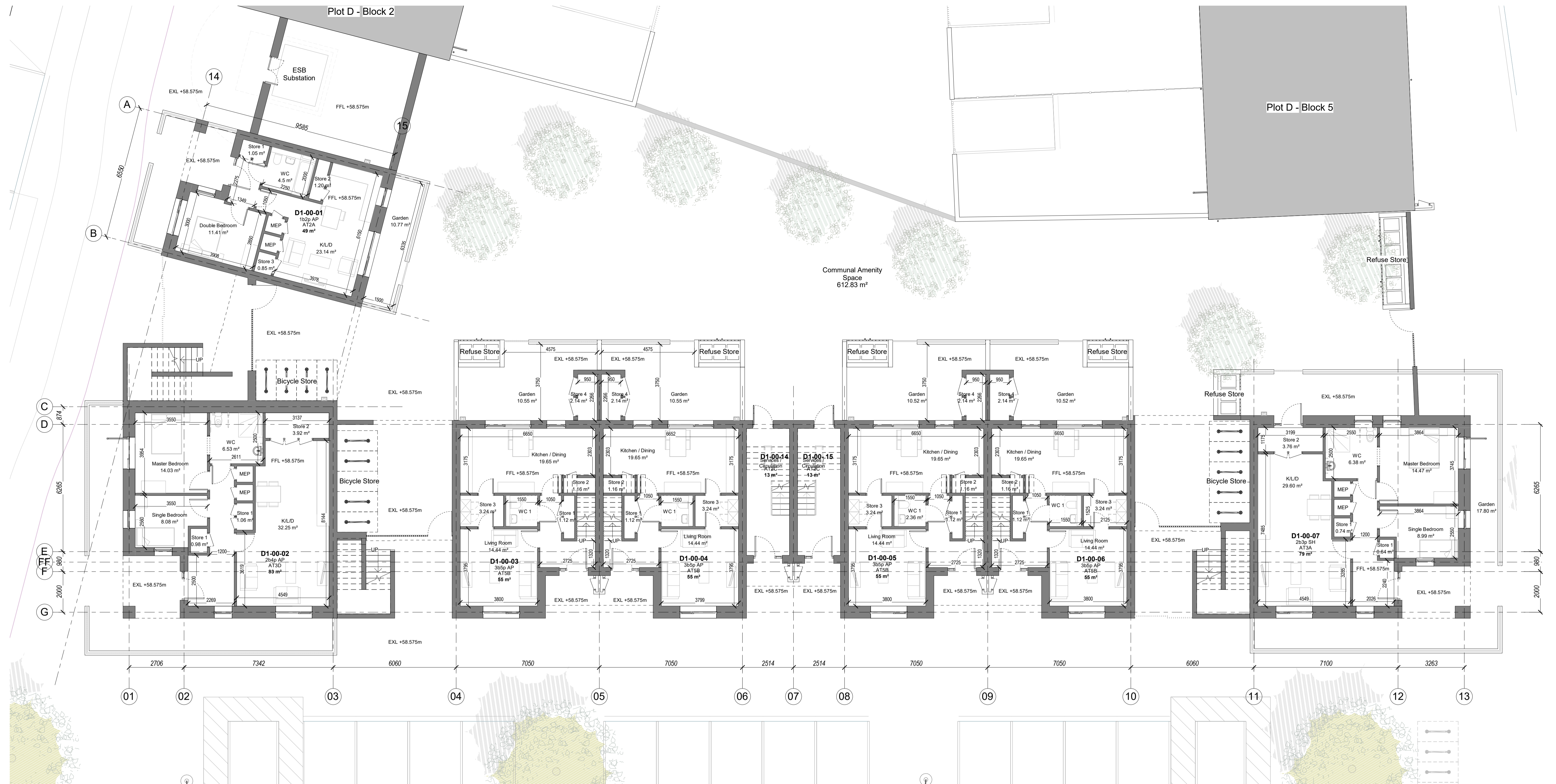
Block D1 - Ground Floor Plan 1:100
