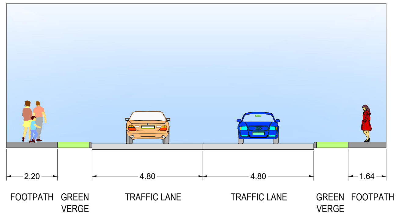
EXISTING CROSS SECTION AT A-A
