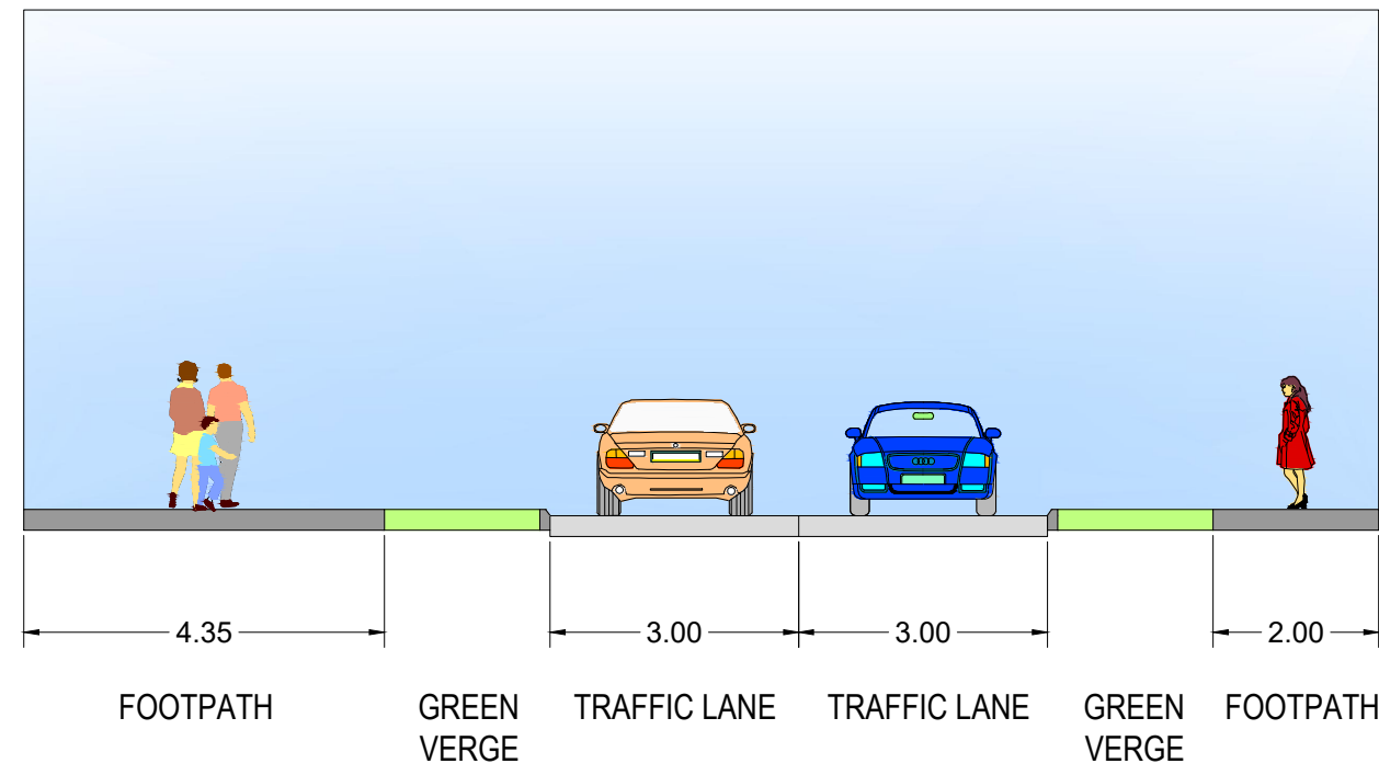
PROPOSED CROSS SECTION A-A
