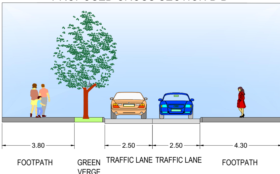
PROPOSED CROSS SECTION B-B
