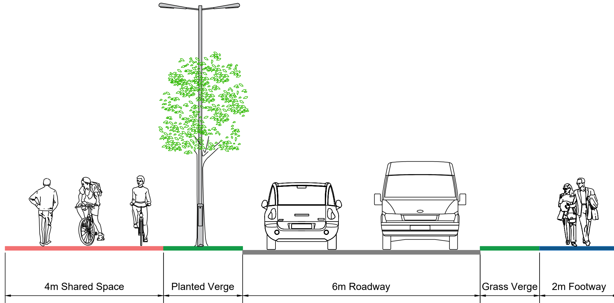
Existing Cross Section
