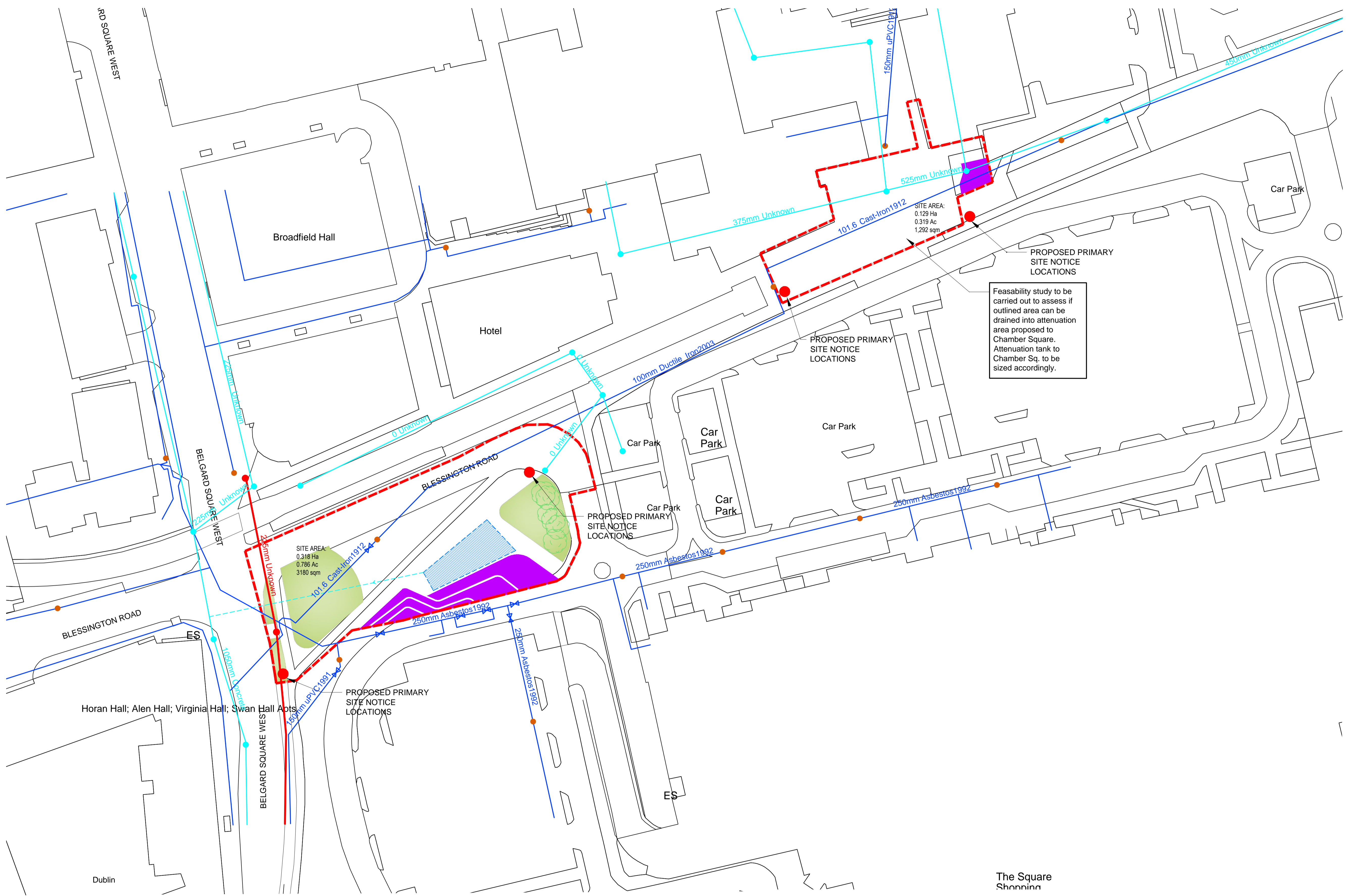
01 PROPOSED DRAINAGE DRAWING/ SITE LOCATION PLAN SCALE = 1:500 @A1, 1:1000@A3
