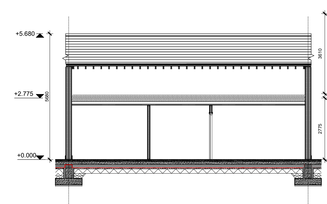
SECTION B-B OF P3
