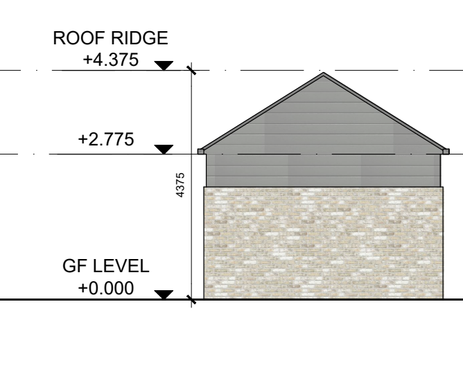
SIDE ELEVATIONS - CCF3 & CCF4
