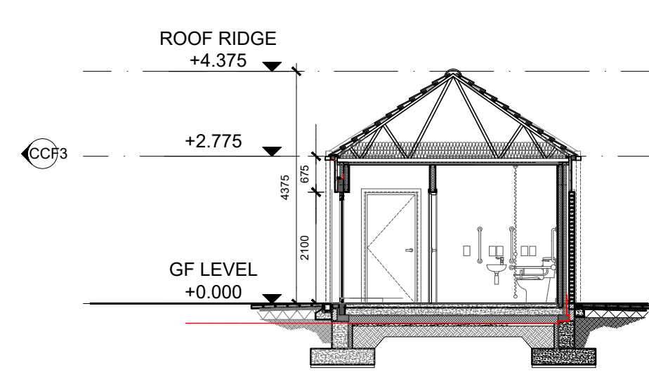
SECTION C-C OF CCF UNIT
