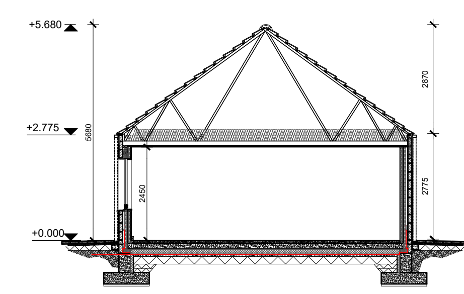
SECTION A-A OF P3
