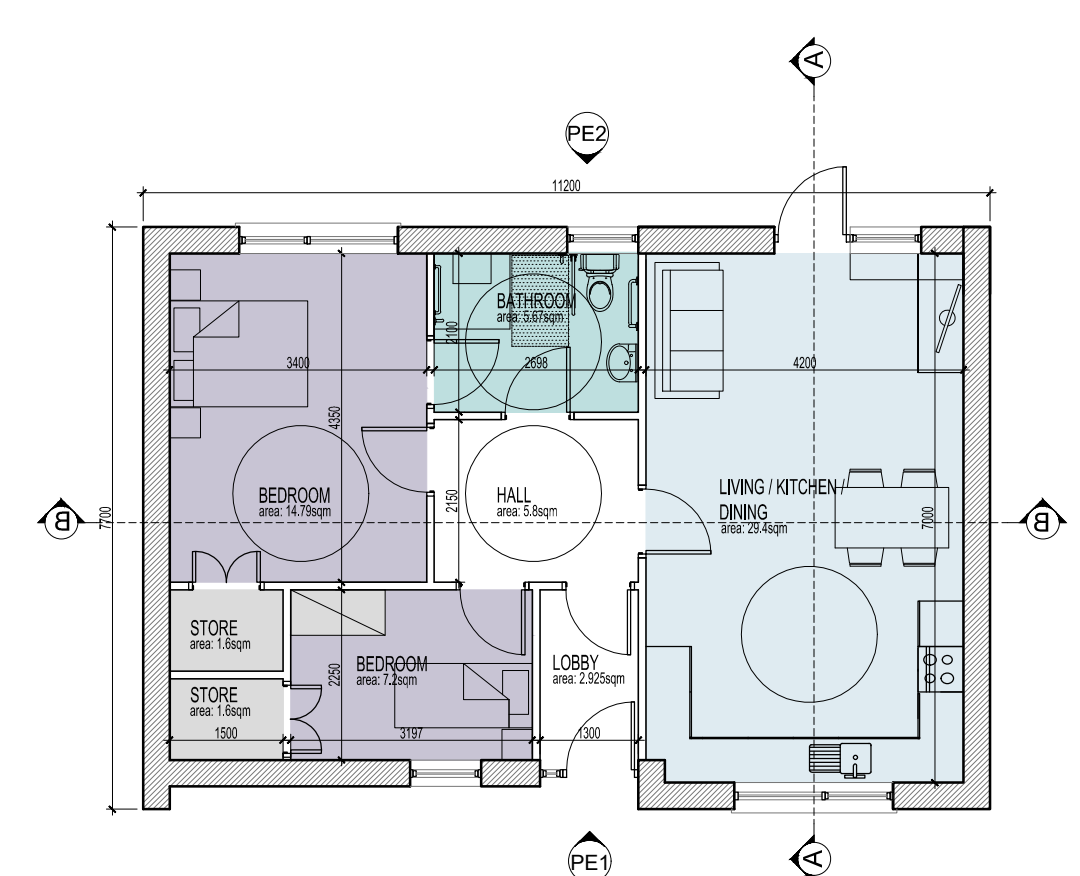
PROPOSED FLOOR PLAN OF CCF UNIT
