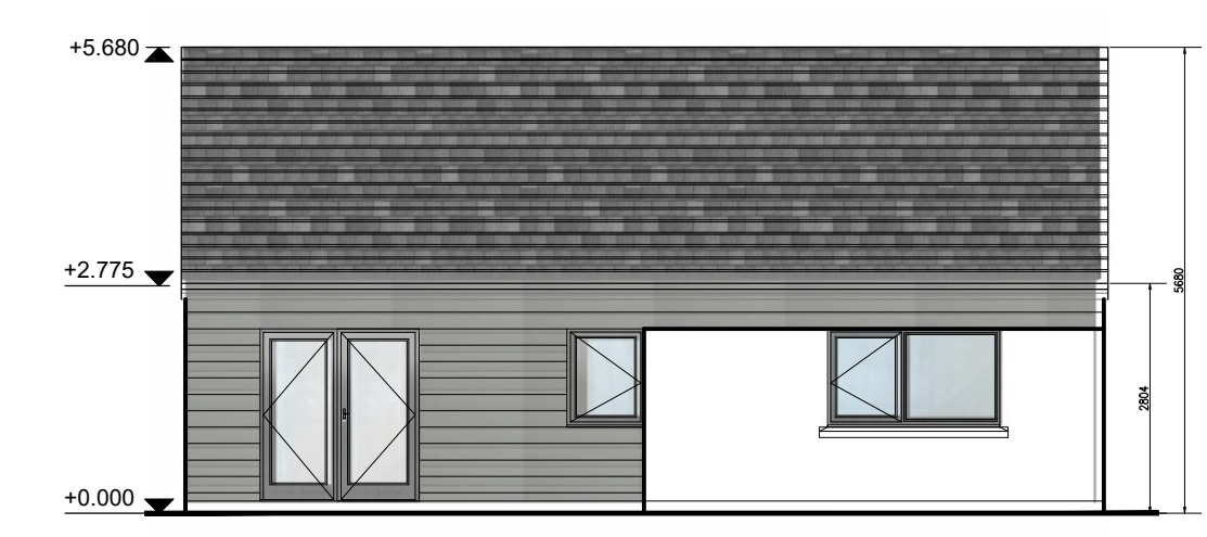
REAR ELEVATION PE2
