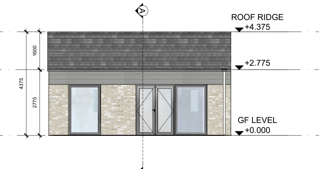
FRONT ELEVATION CCF1
