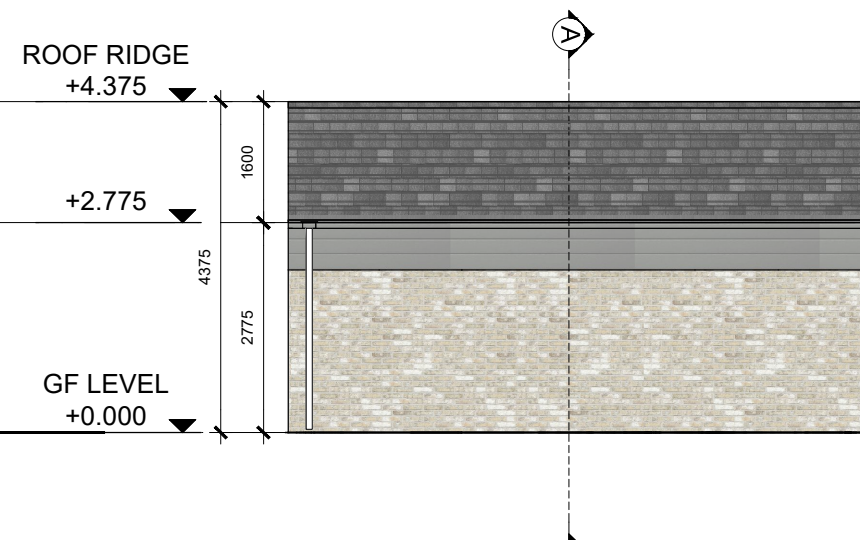
REAR ELEVATION CCF2
