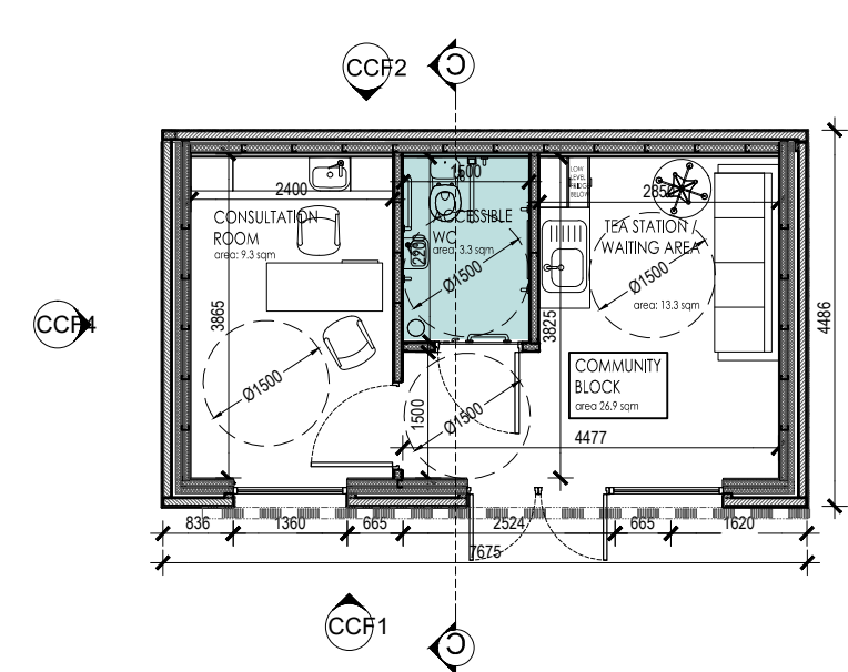
PROPOSED FLOOR PLAN OF CCF UNIT
