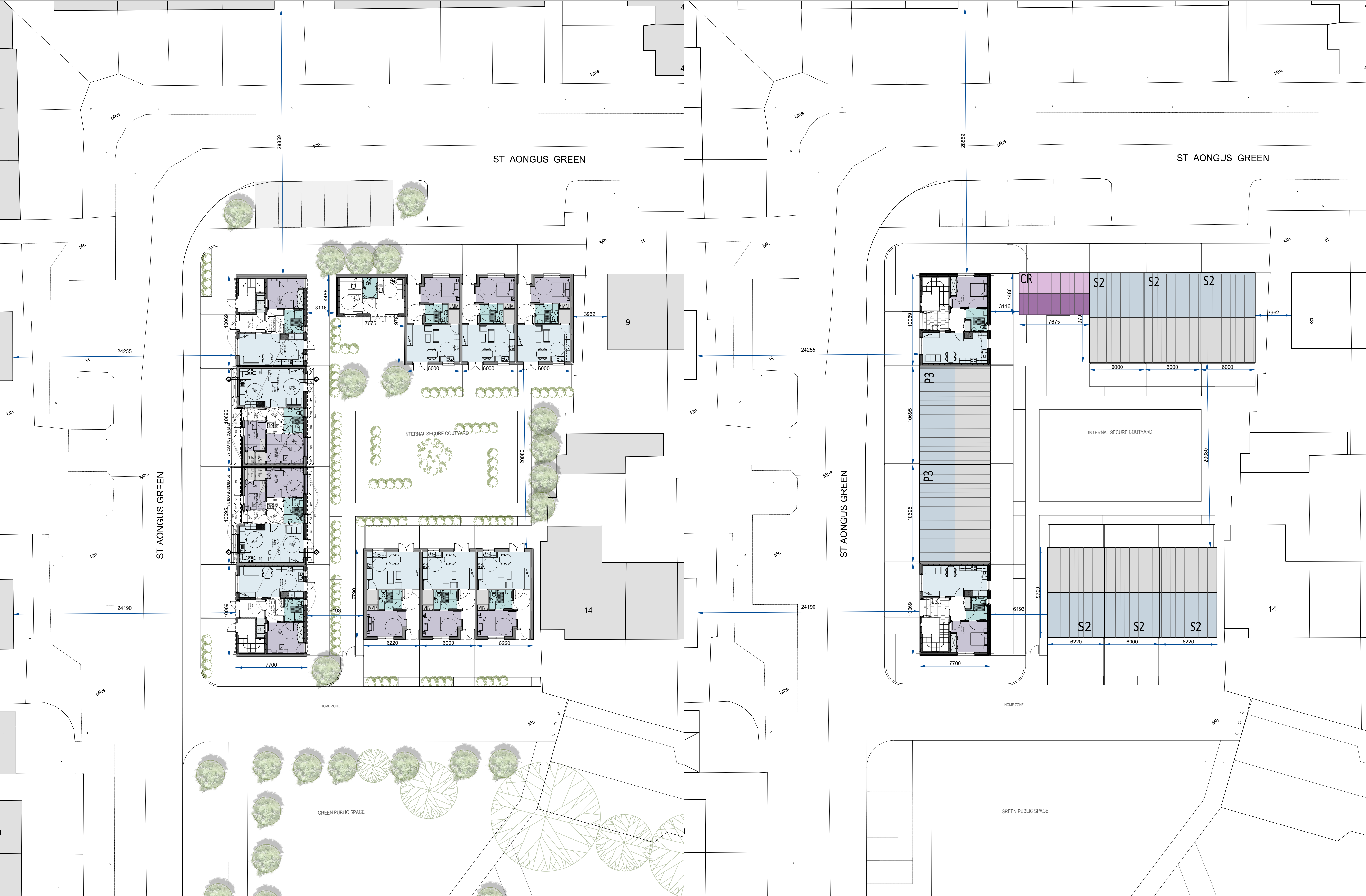
01 s04 PROPOSED GROUND FLOOR PLAN SCALE = 1:200 @A1, 1:400@A3
