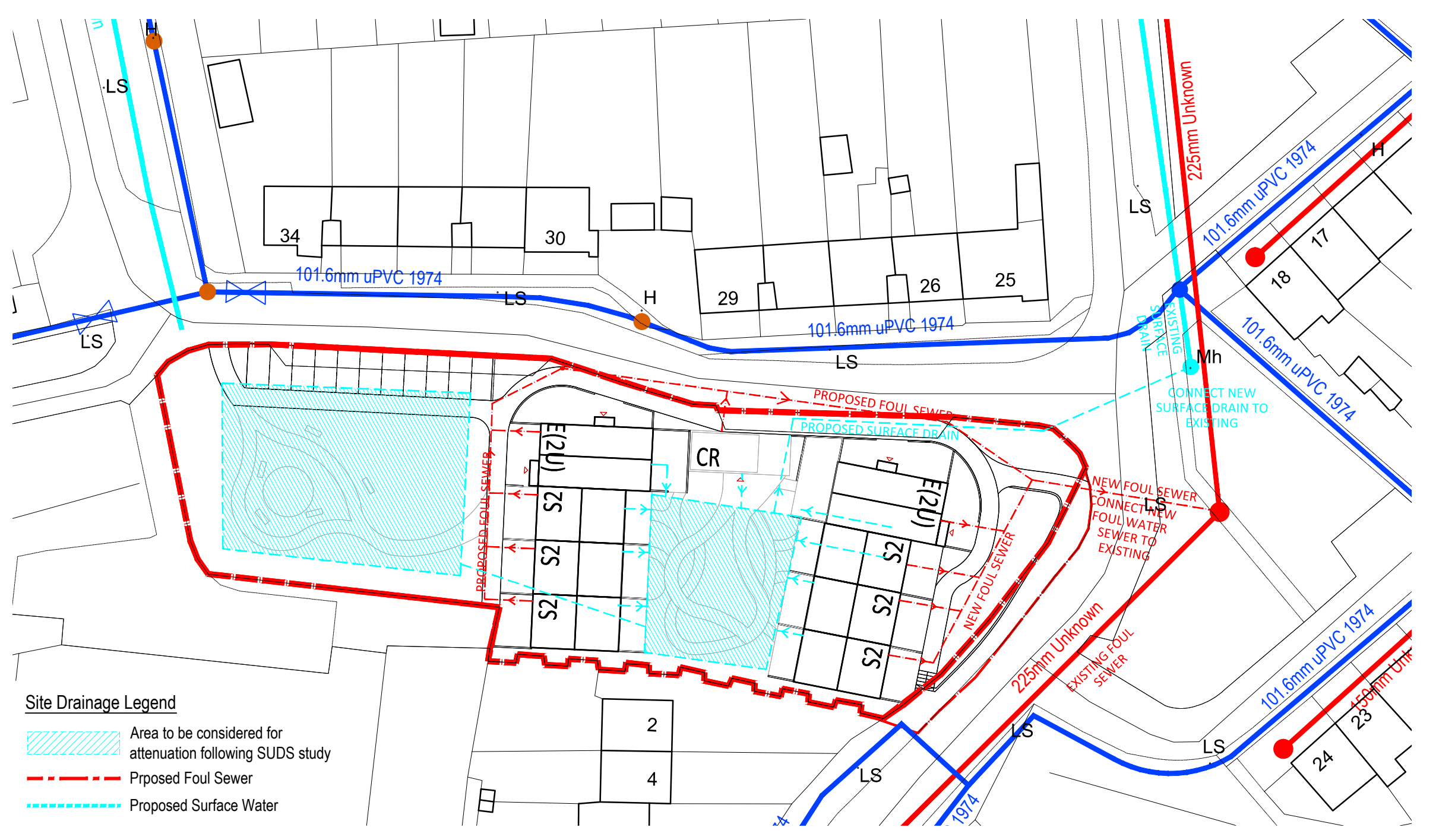
03 PROPOSED DRAINAGE PLAN SCALE = 1:500 @A1, 1:1000@A3
