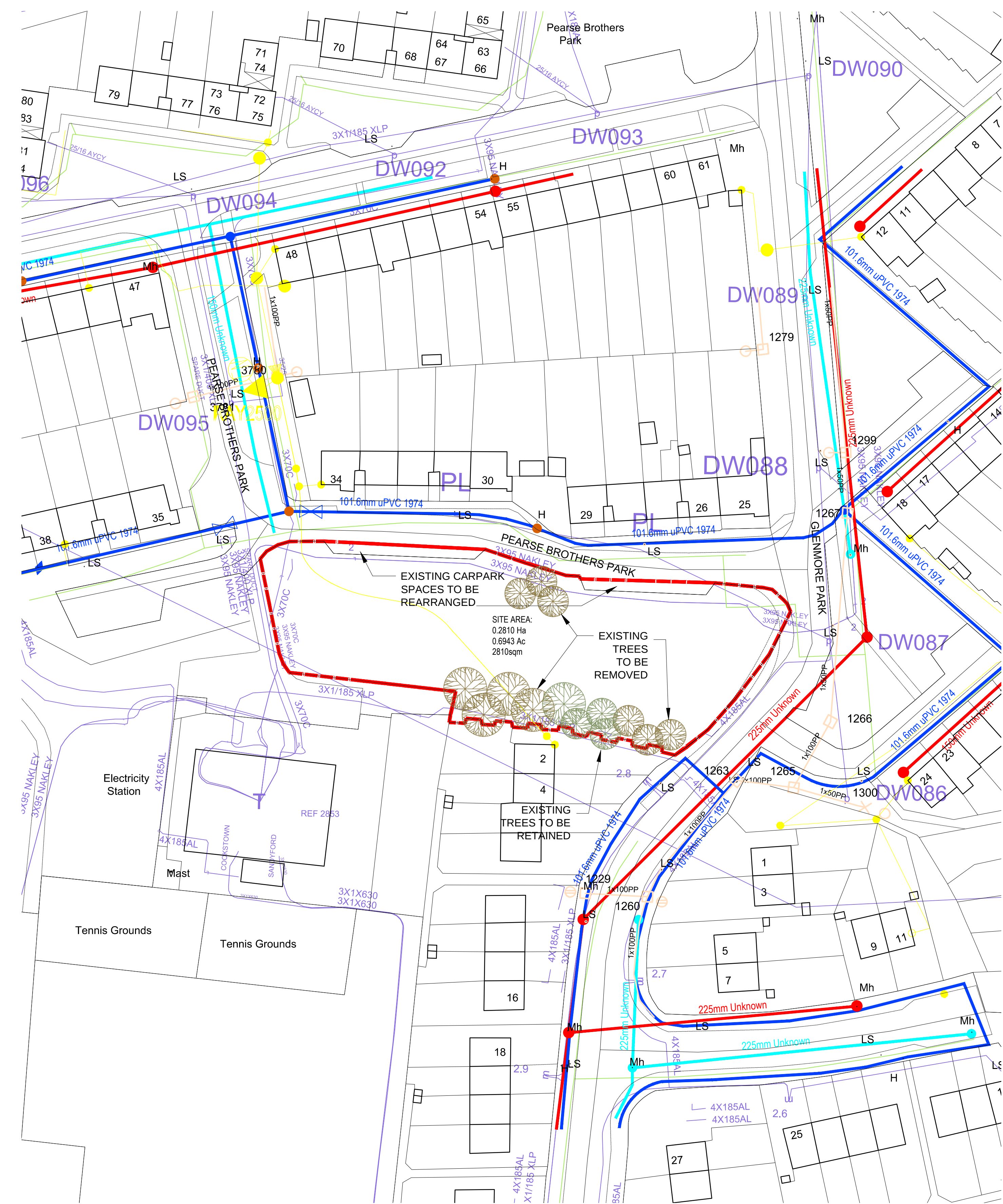
01 CONSTRAINTS PLAN/ EXISTING SITE PLAN SCALE = 1:500 @A1, 1:1000@A3
