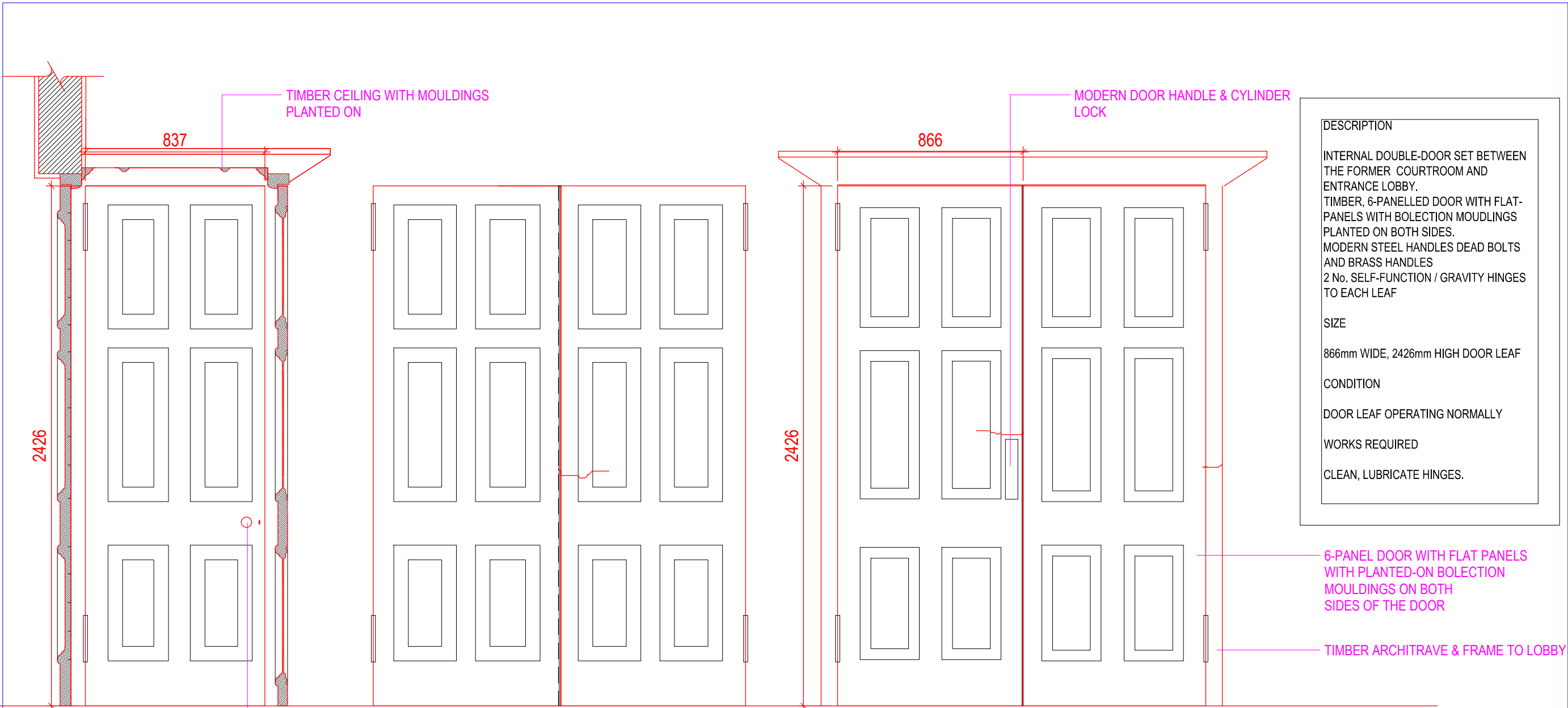
SECTION
