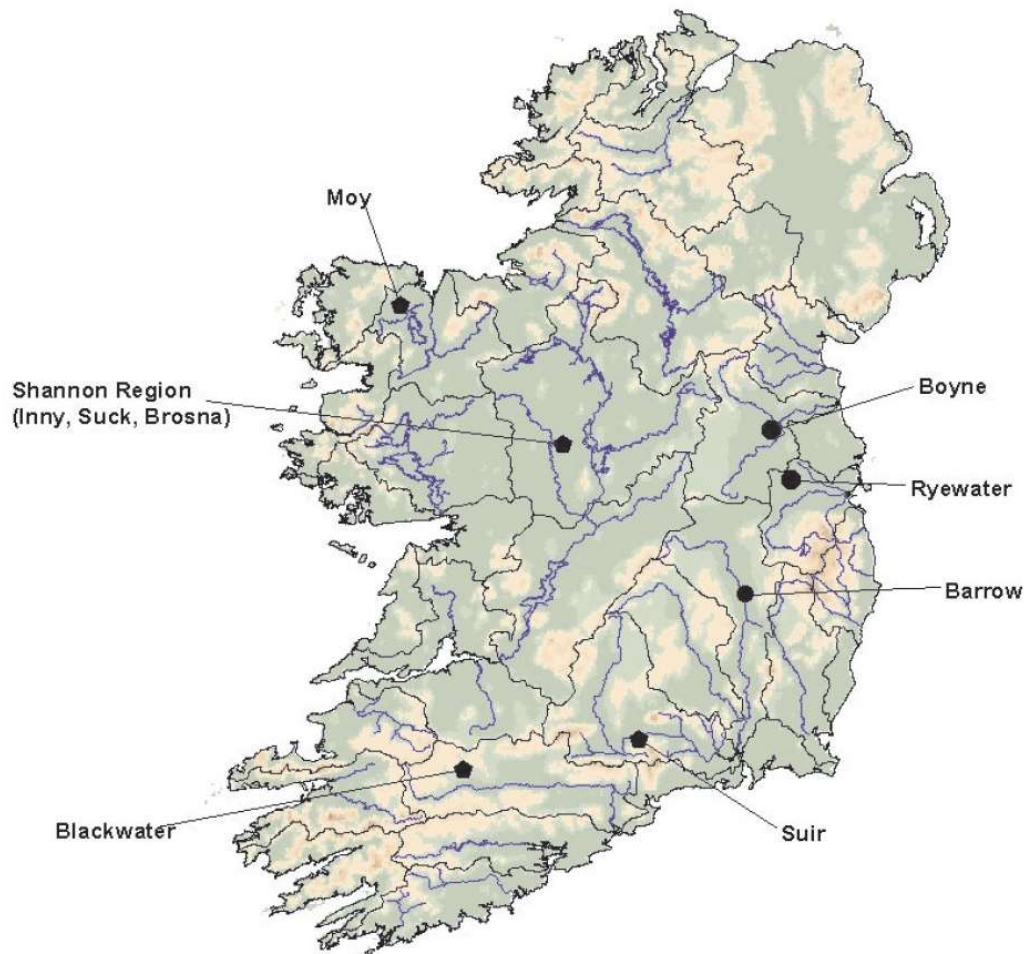
Figure 1-1 Location of the study catchment used in Maynooth (2008)
