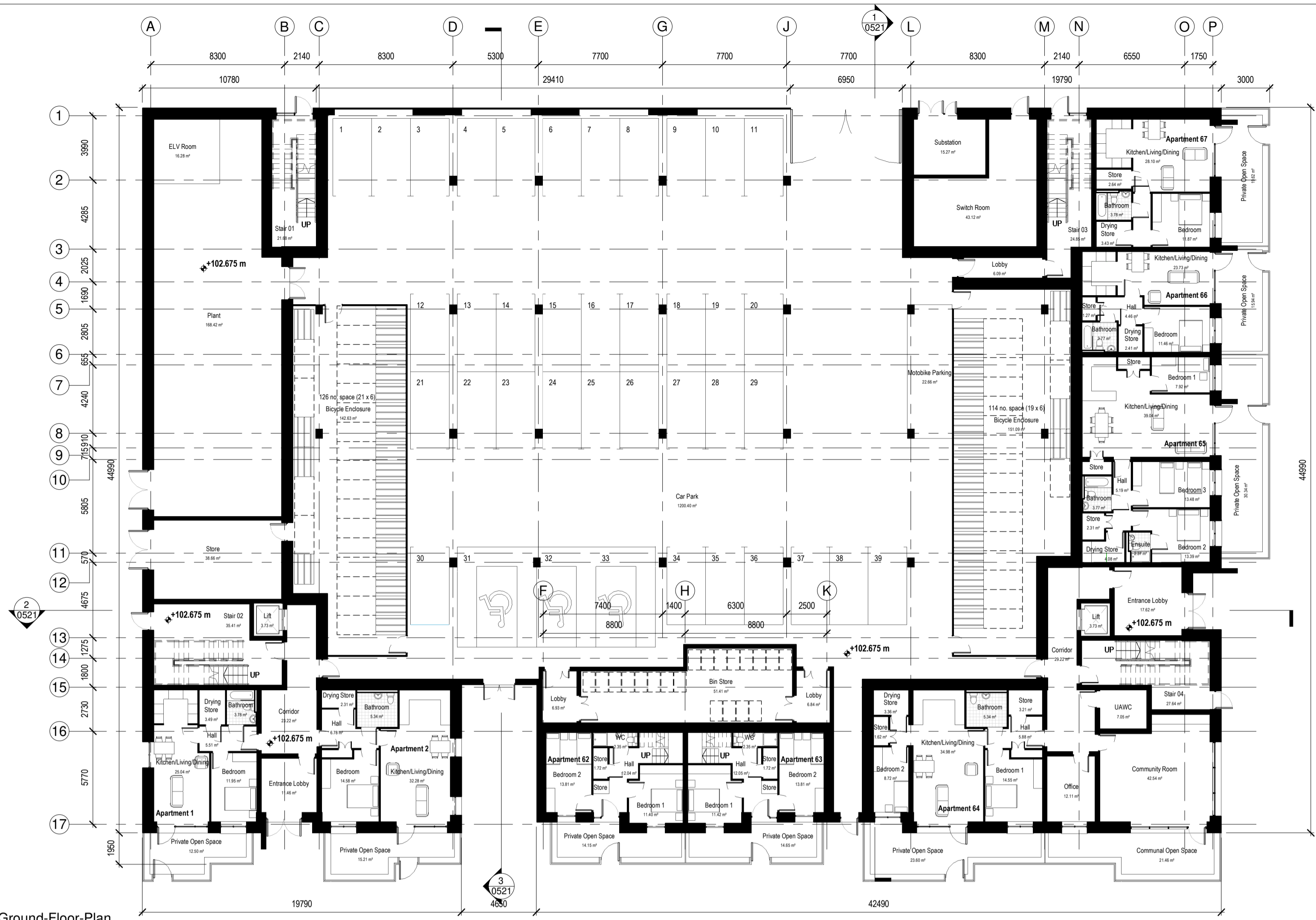
1 Planning-00-Ground-Floor-Plan T: 200
