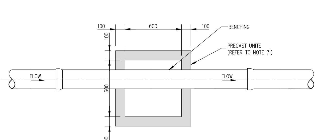
PLAN INSPECTION CHAMBER (PRECAST CONCRETE CONSTRUCTION)
