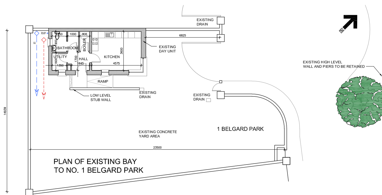
02 01 PLANS TO EXISTING BAY NOS 1 & 10 1:100@A1 1:200@A3
