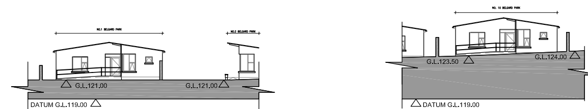
02 02 SITE SECTION OF EXISTING BAY NOS 1 & 10 1:200@A1 NTS@A3
