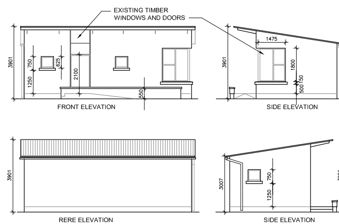
TYPICAL ELEVATIONS OF EXISTING BAYS TO BELGARD PARK
