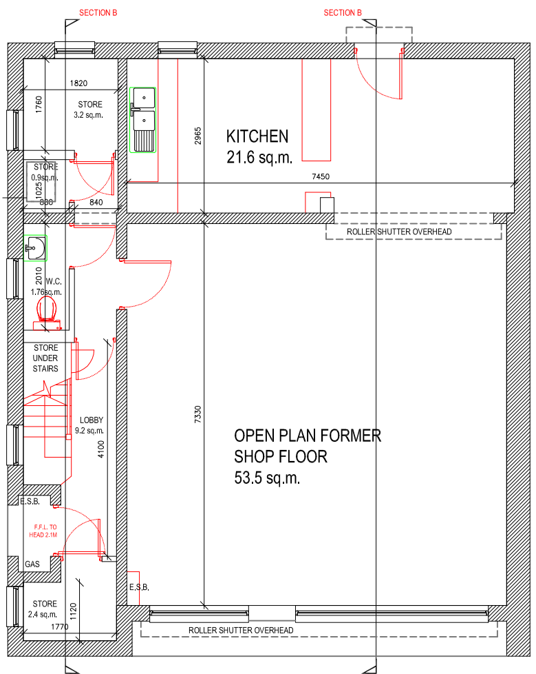
GROUND FLOOR PLAN SCALE 1:100 99.0 sq.m.
