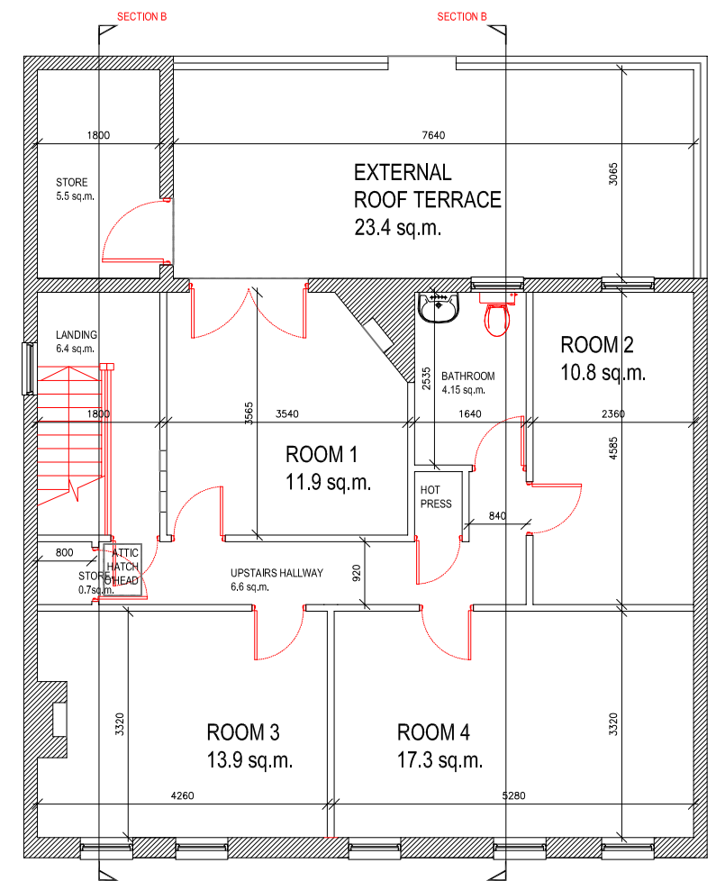
FIRST FLOOR PLAN SCALE 1:100 77.1 sq.m. plus 9.6 sq.m. on ground floor
