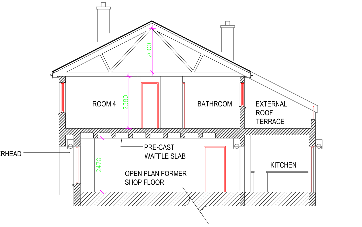
SECTION B SCALE 1:100
