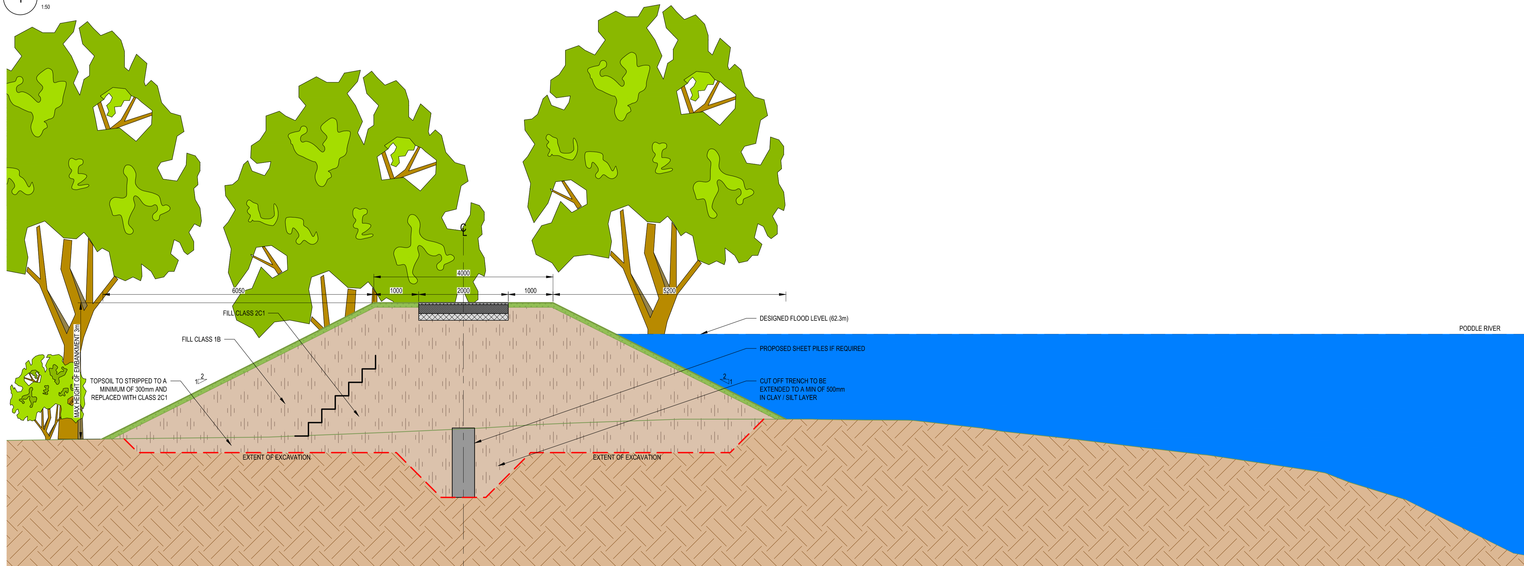
2 Proposed Embankment & Drain Typical Section - Flood
