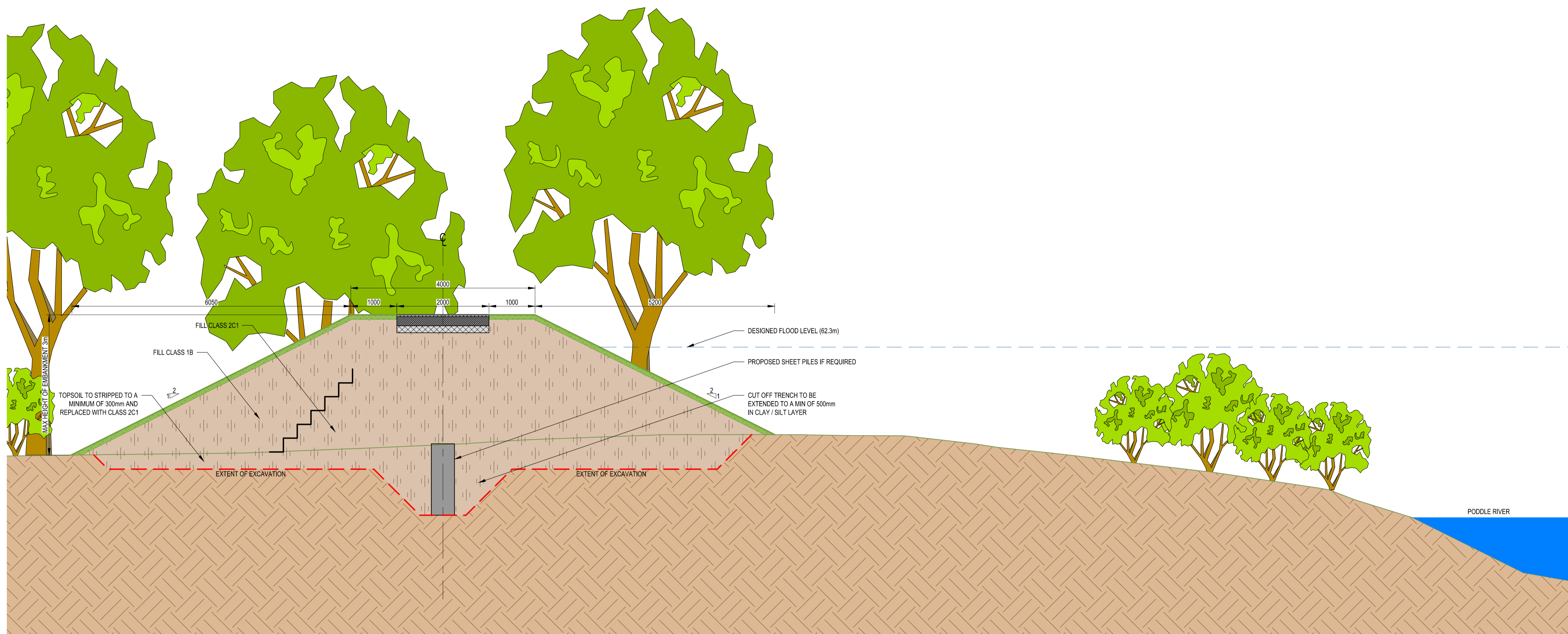
1 Proposed Embankment & Drain Typical Section - Normal
