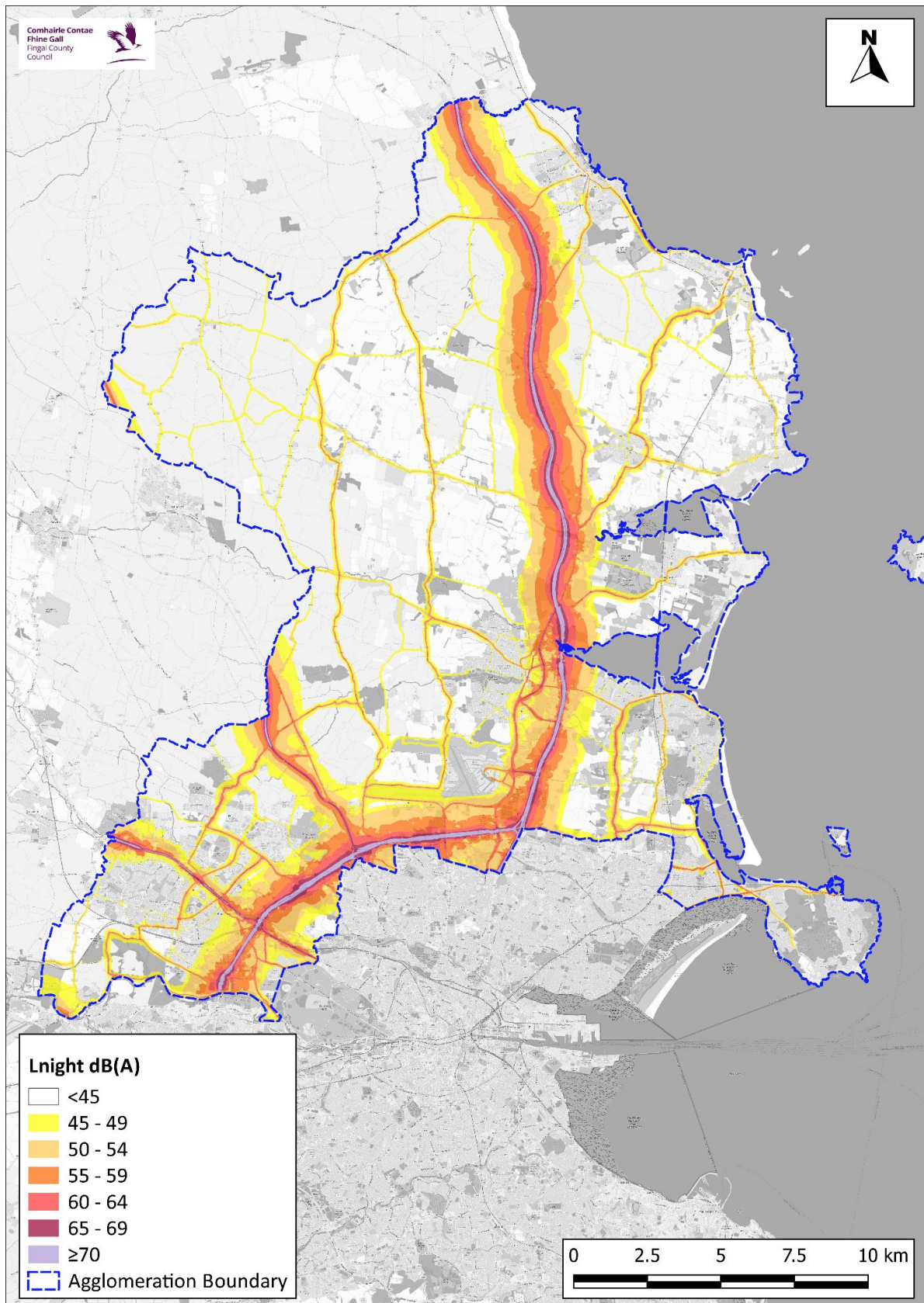
Figure 6 - 2017 Noise Exposure Map – All Roads L_{\text{night}} dB(A) FCC
