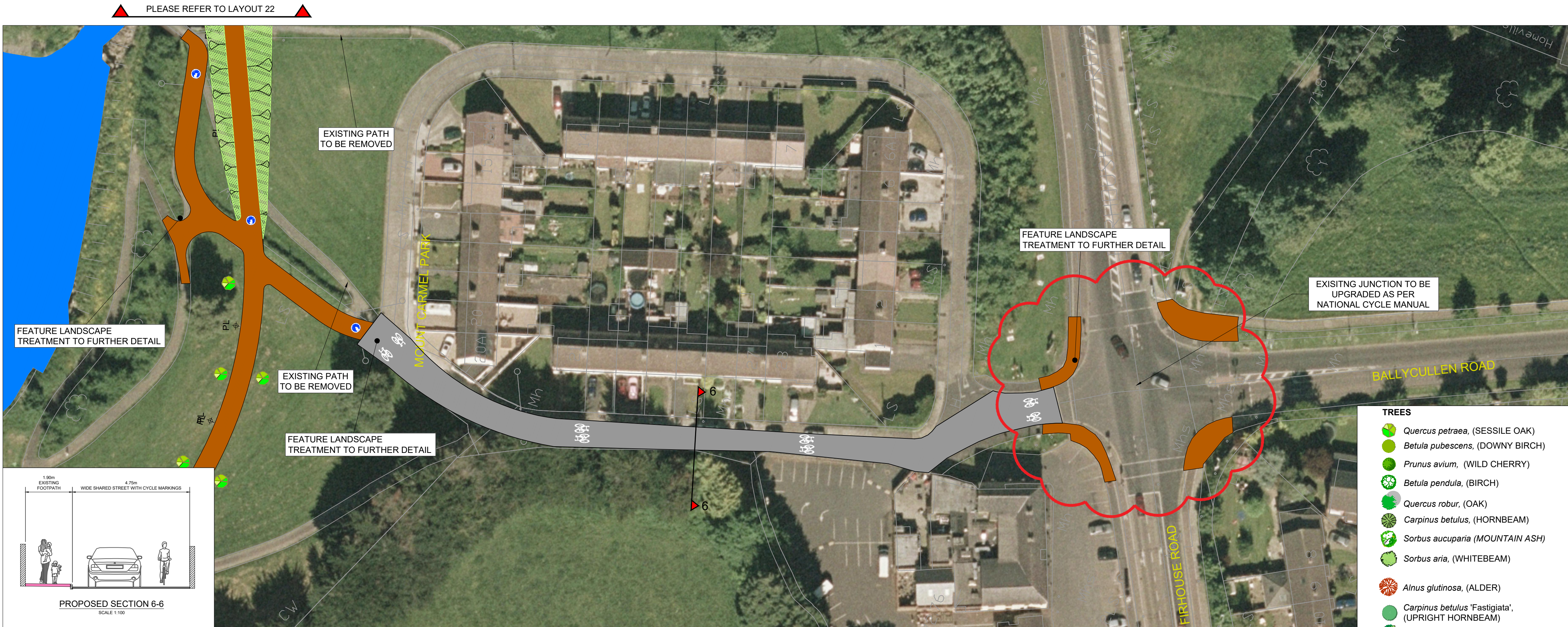
LAYOUT - 21 SCALE: 1:500 PLEASE REFER TO LAYOUT 20
