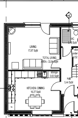
HOUSE TYPE K5
