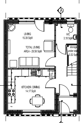
HOUSE TYPE K4
