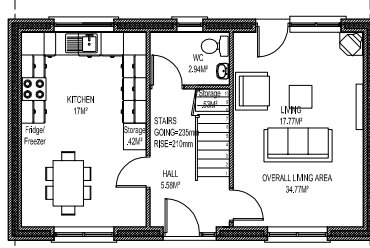
HOUSE TYPE B5
