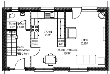
HOUSE TYPE B4
