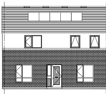
HOUSE TYPE B4
