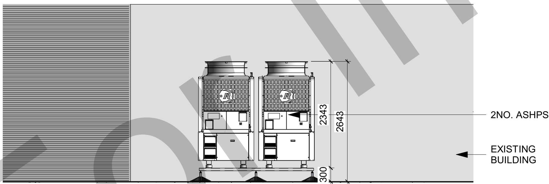
Rua Red Art Centre - Section 01 1 : 50
