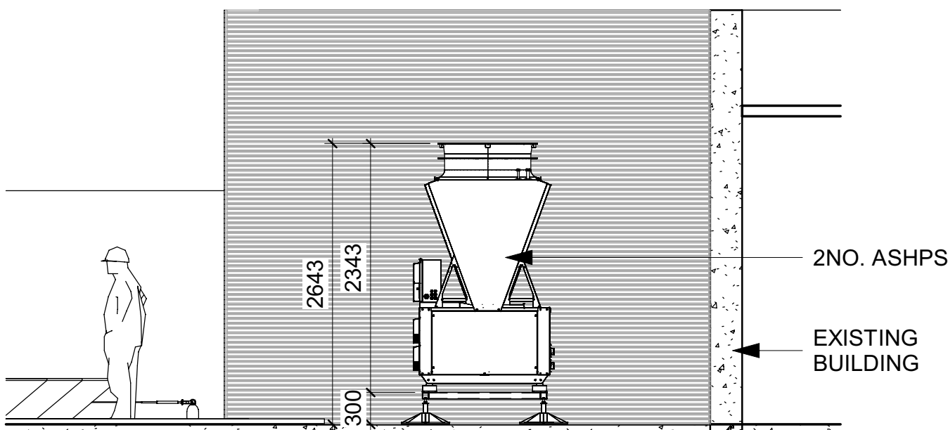
Rua Red Art Centre - Section 02 1 : 50
