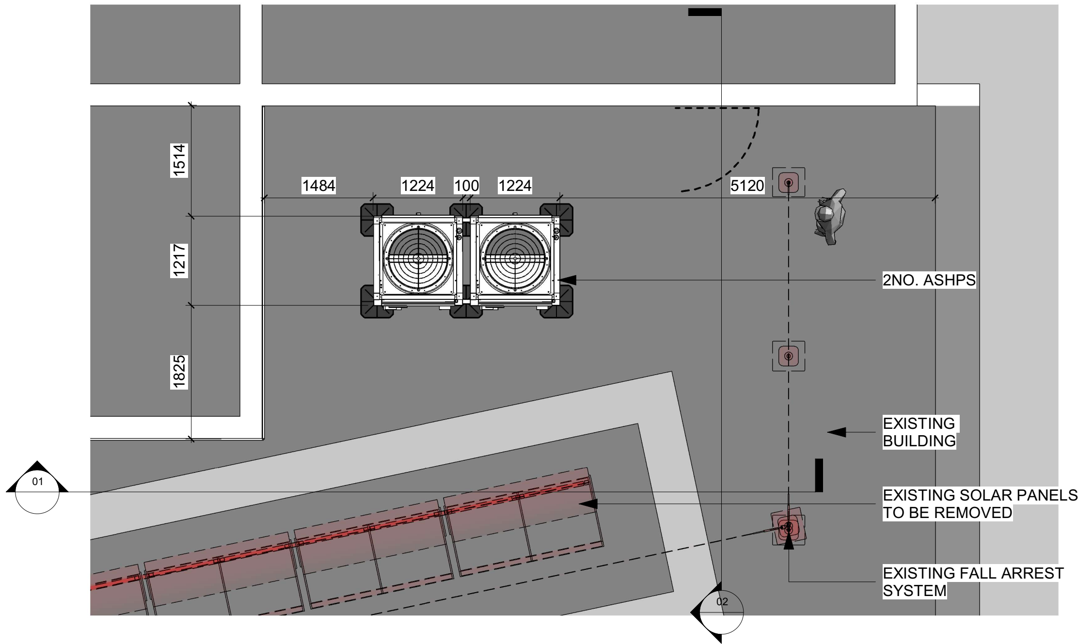
Rua Red Art Centre- Site Plan (Detailed) Copy 1 1 : 50
