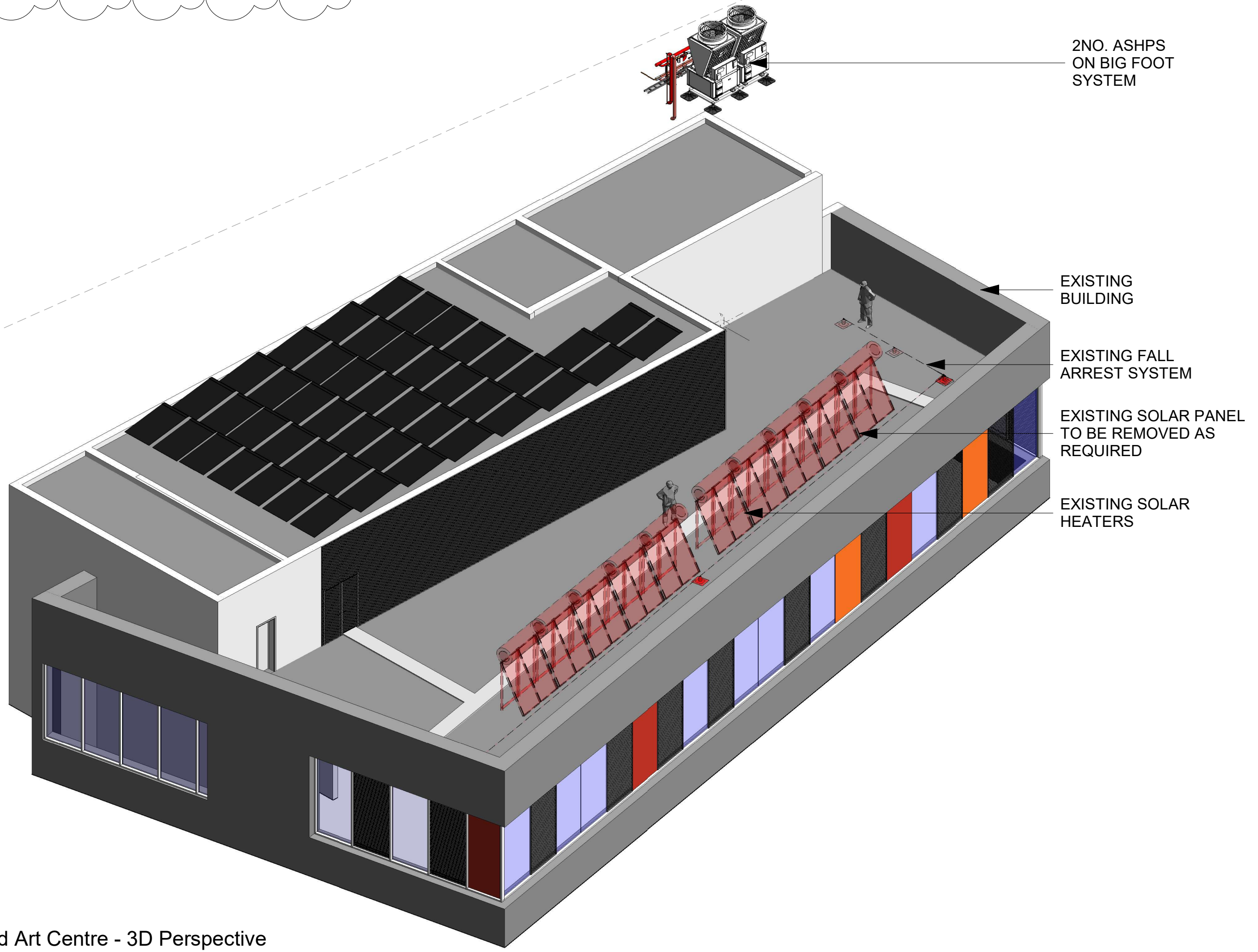
Rua Red Art Centre - 3D Perspective
