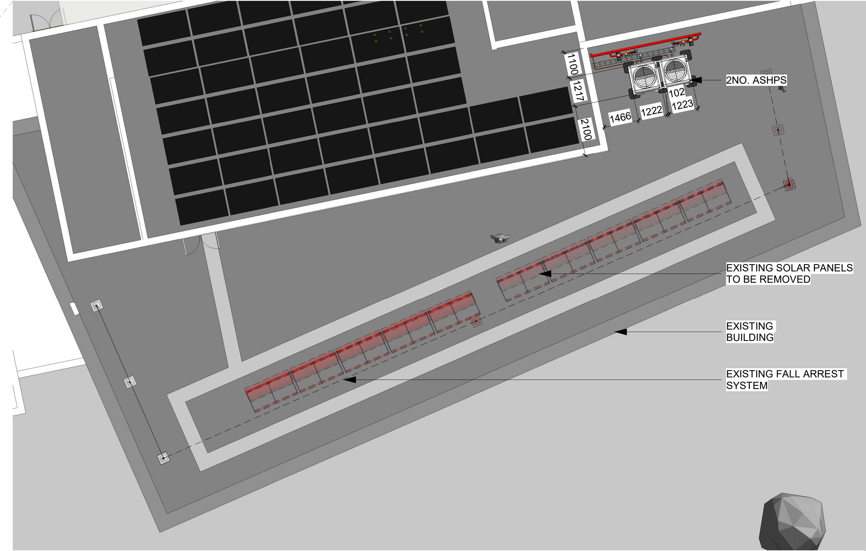
Rua Red Art Centre- Site Plan (Detailed) 1 : 100
