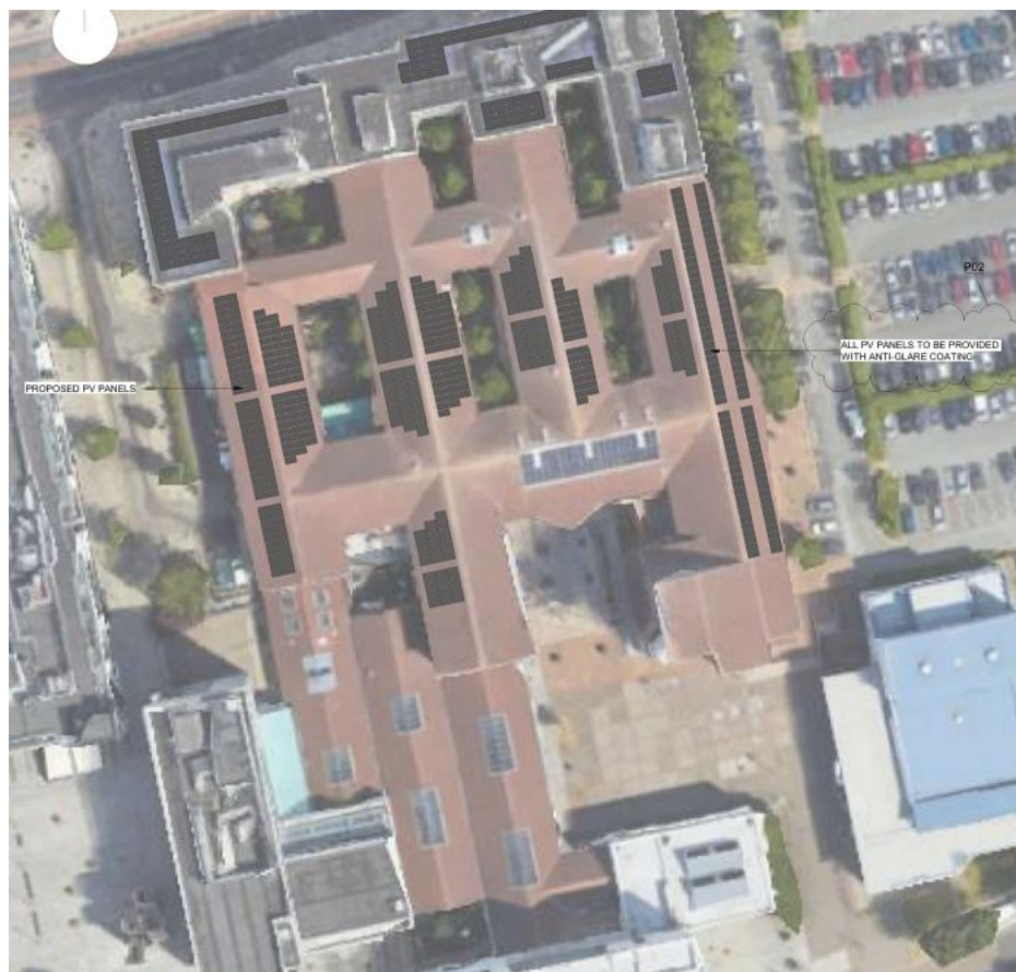
Figure 3: Proposed solar PV array to be installed on the building roof
