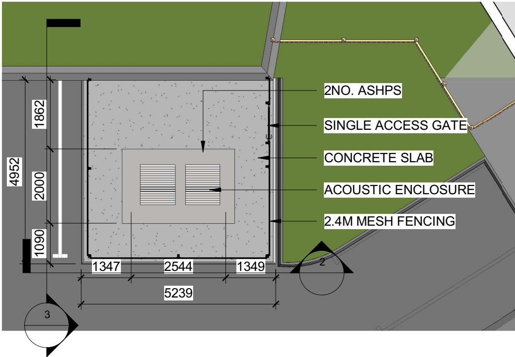
Clondalkin Civic Offices - Compound Plan View 1 : 100
