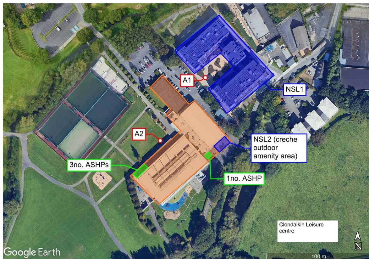
Figure 2: Site Location, NSL Locations and Measurement Locations.
