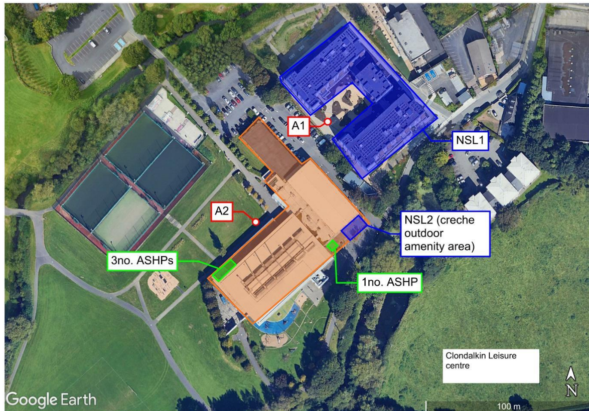
Figure 1: Site Location, Measurement Location A1 and A2, Noise Sensitive Locations (NSL), and the Surrounding Area.
