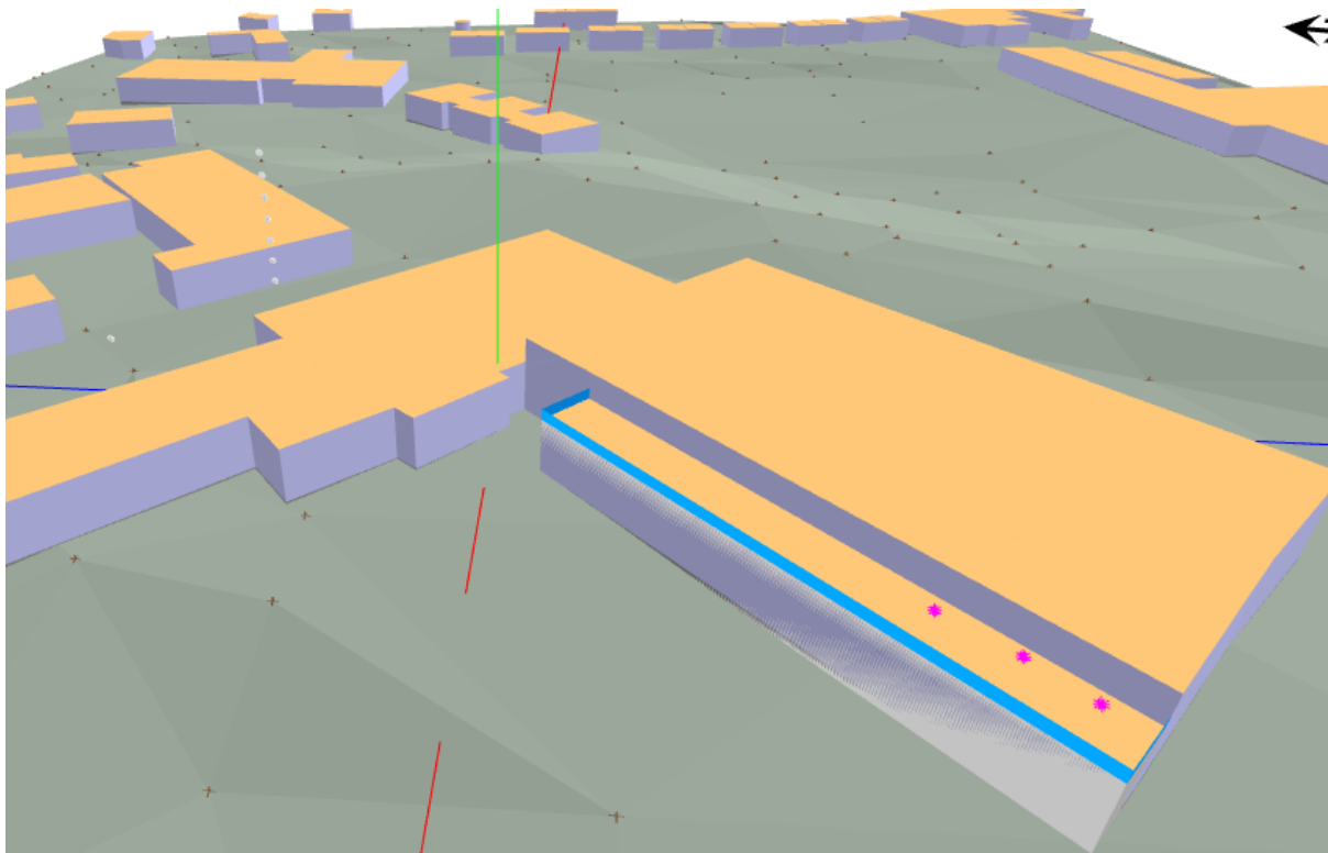
Figure 5: SoundPLAN 9.1 Model of the Proposed Development.
