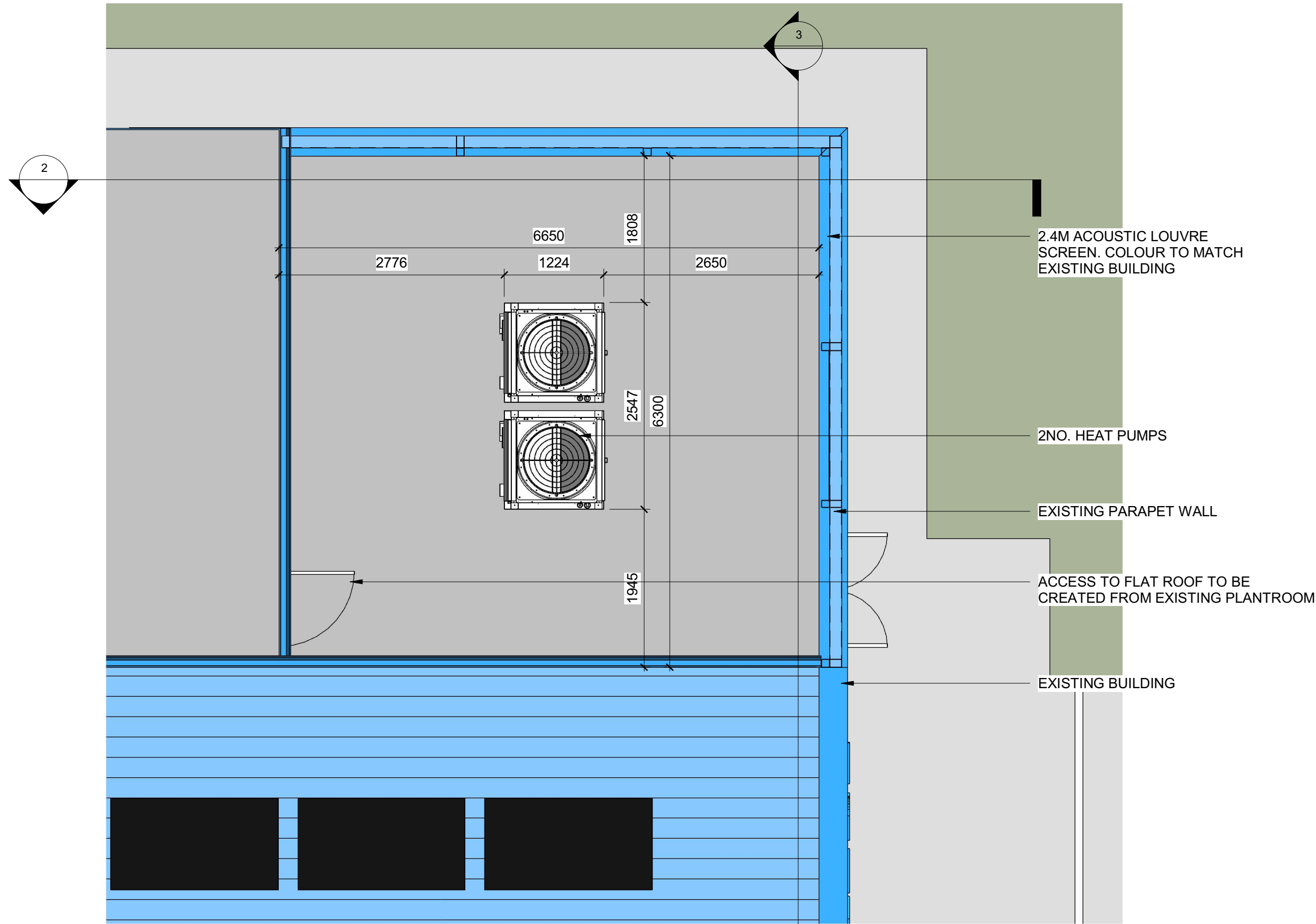
Civic Theatre - Site Plan (Detailed) 1 : 50
