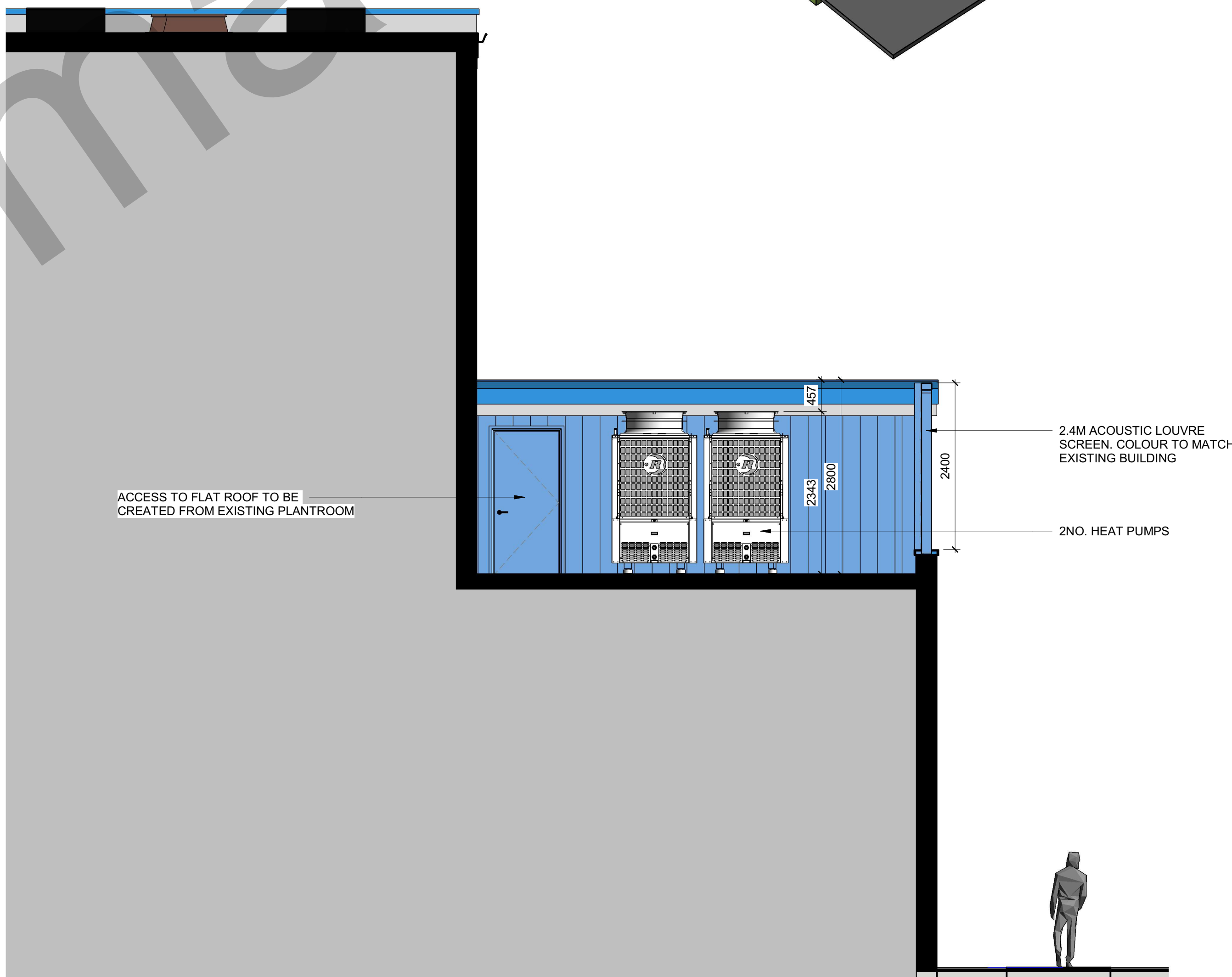
Civic Theatre - Section 02 1 : 50
