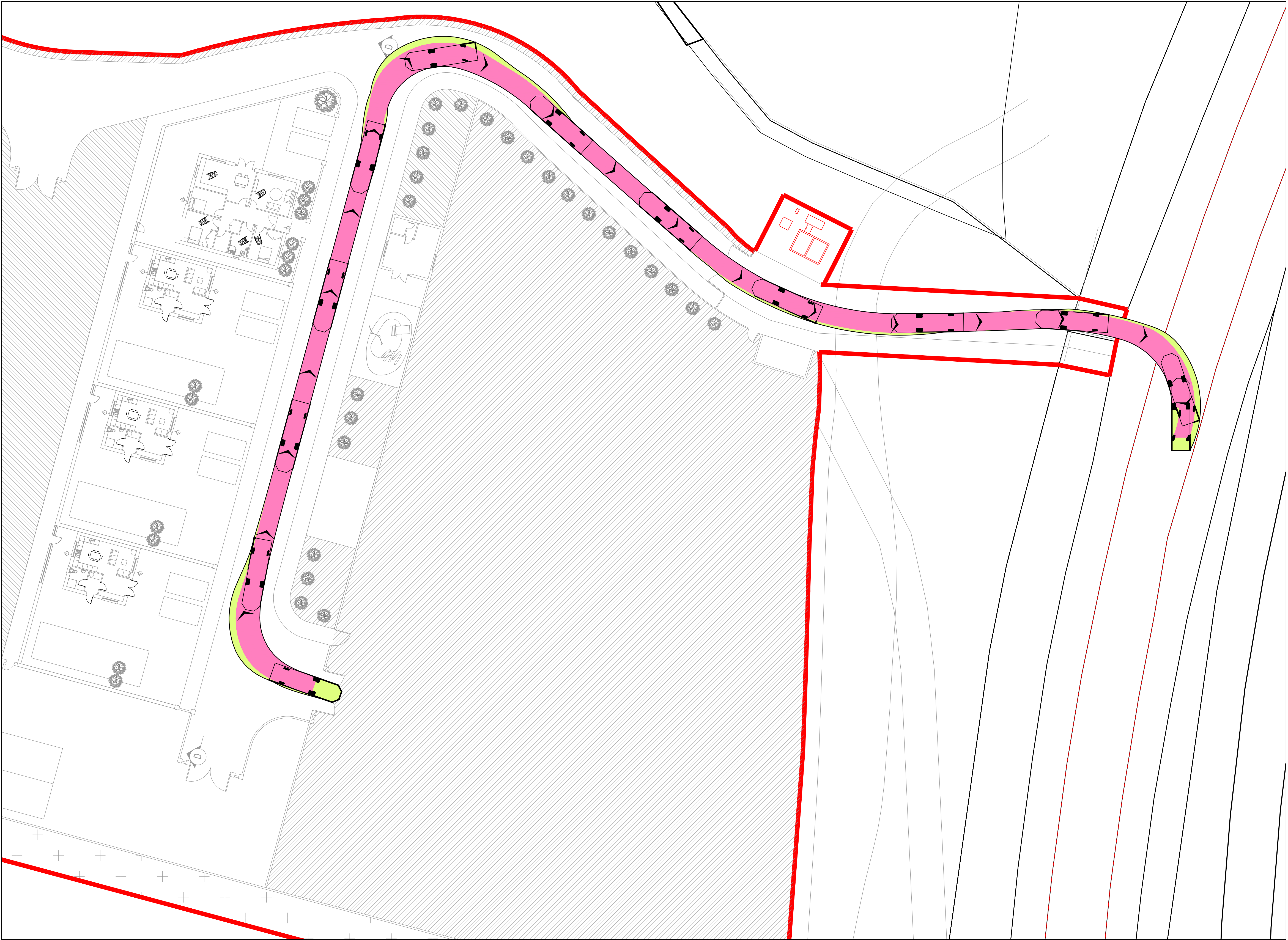
Auto Track Analysis - Fire Appliance Out SCALE 1:250
