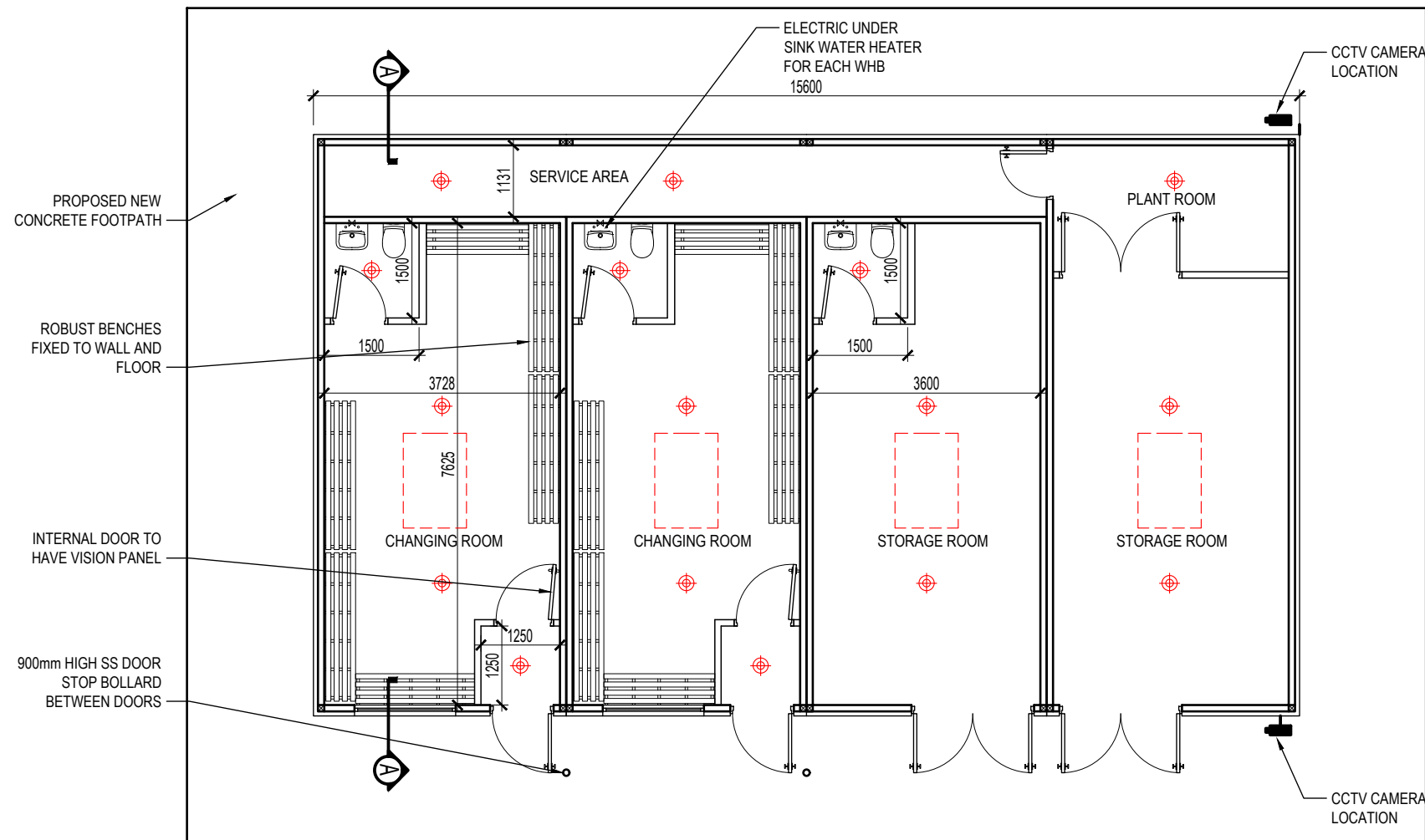
TYPICAL 4 BAY PLAN
