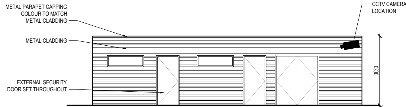
TYPICAL FRONT ELEVATION
