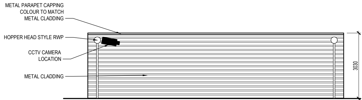
TYPICAL REAR ELEVATION
