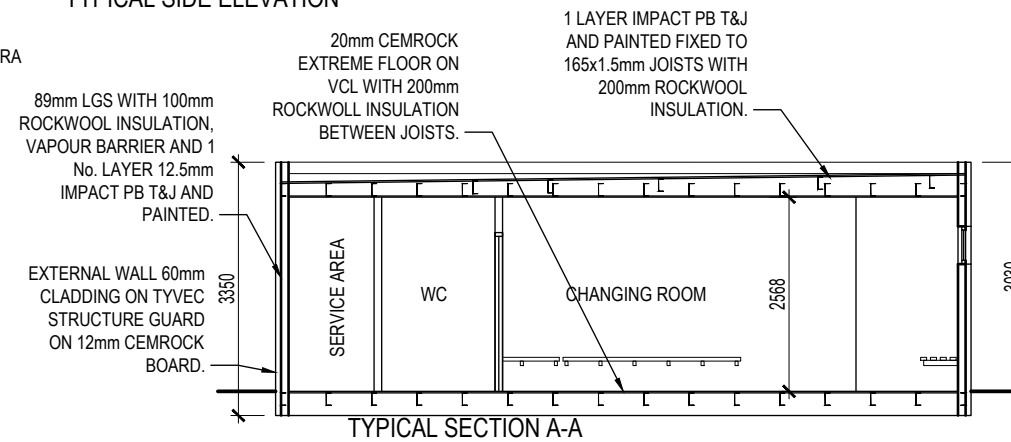
TYPICAL SECTION A-A
