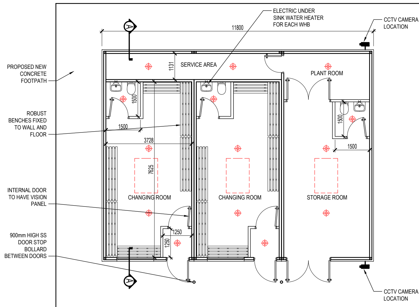
TYPICAL 3 BAY PLAN
