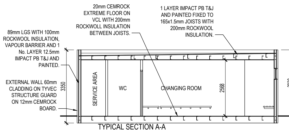
TYPICAL SECTION A-A
