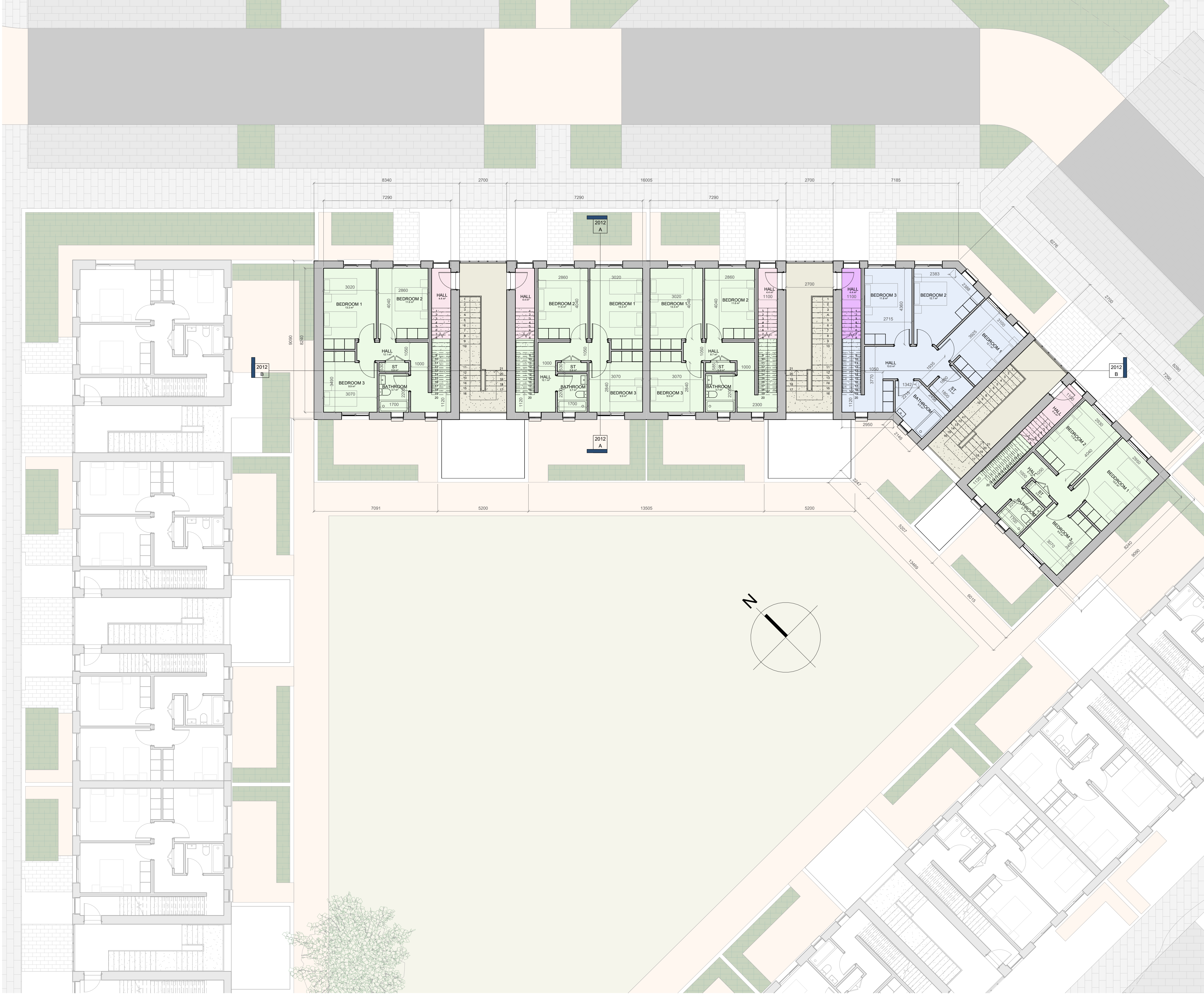
KEY PLAN 1:2000
