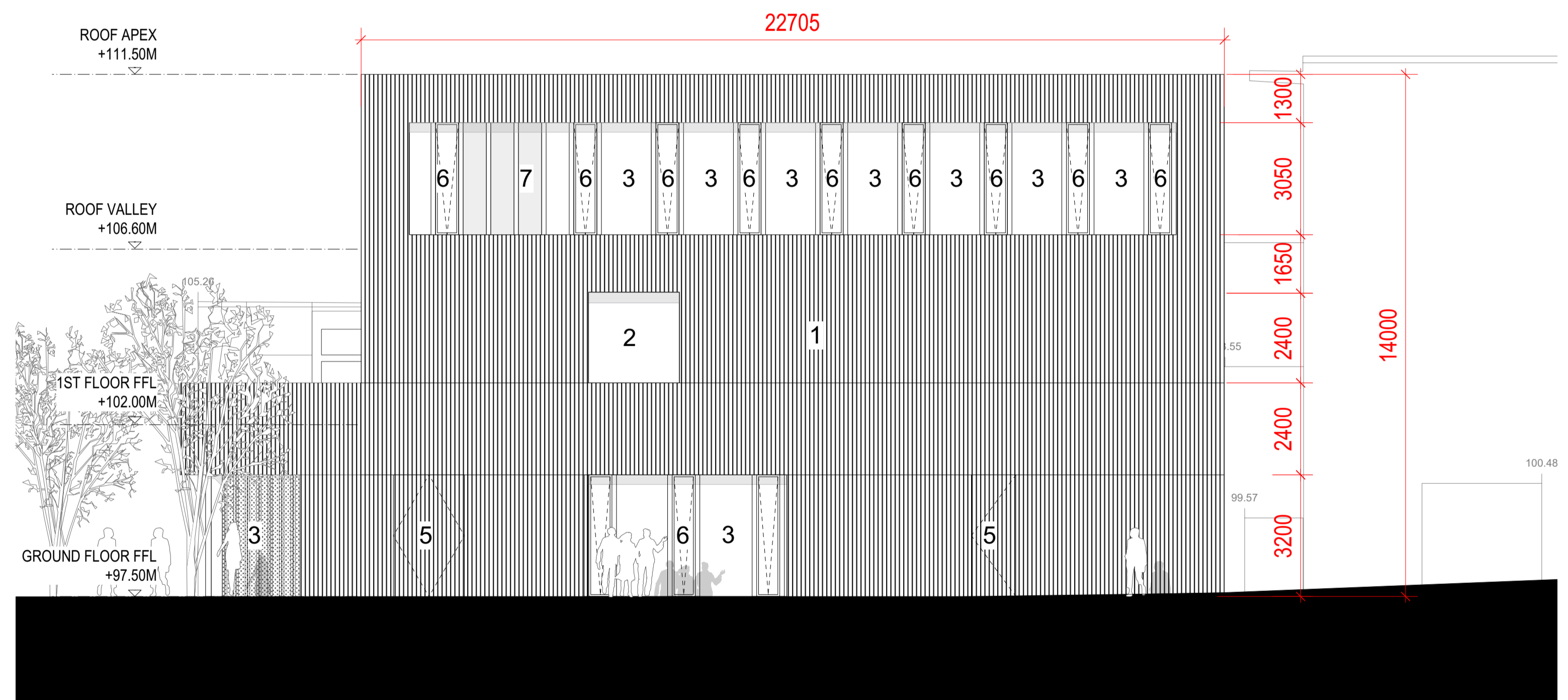
1 East Elevation - Proposed 113 1:100@A1
