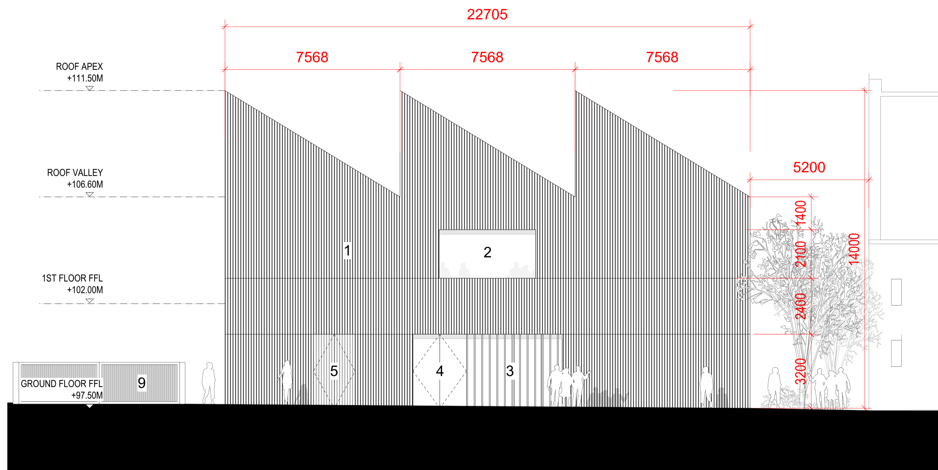
1 North Elevation - Proposed 112 1:100@A1
